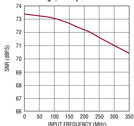
LTC2171-14: SNR vs Input Frequency, -1\text{dBFS} , 2\text{V} Range, 40\text{Mps}
