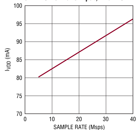
LTC2171-14: I_{VDD} vs Sample Rate, 5\text{MHz} Sine Wave Input, -1\text{dBFS}
