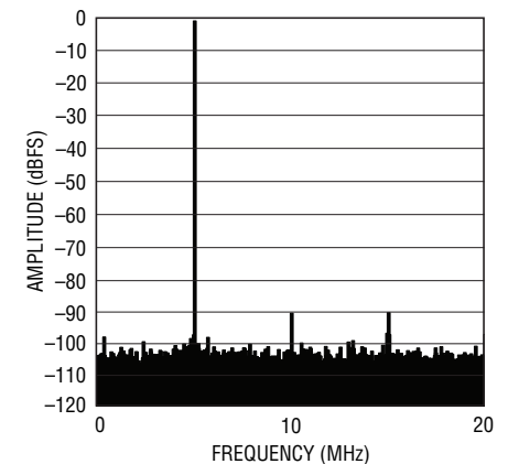
LTC2171-14: 8k Point FFT, f_{IN} = 5\text{MHz} -1dBFS, 40Mps
