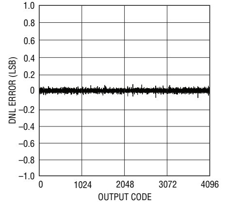
LTC2173-12: Differential Nonlinearity (DNL)
