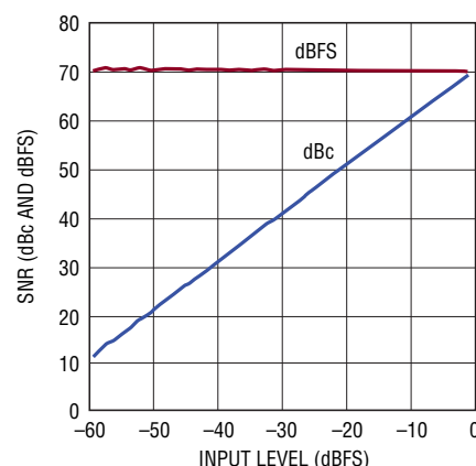
LTC2175-12: SNR vs Input Level, f_{IN} = 70\text{MHz} , 2V Range, 125Msps
