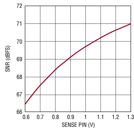
LTC2175-12: SNR vs SENSE, f_{IN} = 5\text{MHz} , -1dB
