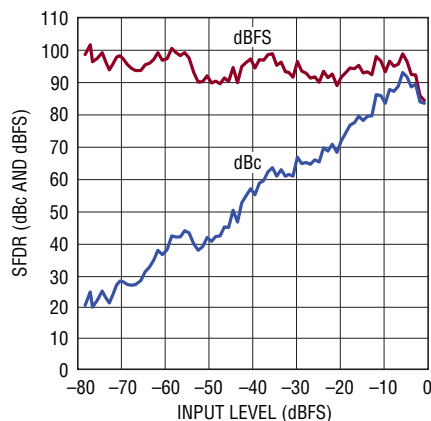
LTC2175-12: SFDR vs Input Level, f_{IN} = 70\text{MHz} , 2V Range, 125Msps
