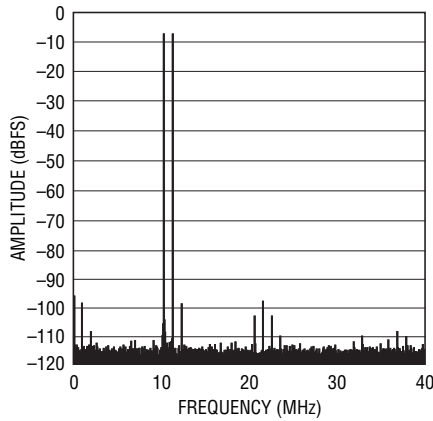
LTC2193: 64k Point, 2-Tone FFT, f_{IN} = 69\text{MHz} , 70\text{MHz} , -7\text{dBFS} , 80\text{Mpsps}
