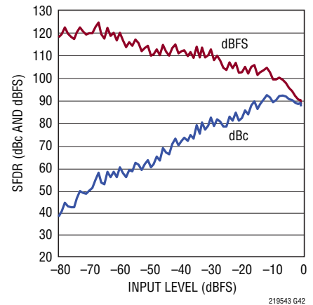
LTC2193: SFDR vs Input Level, f_{IN} = 70\text{MHz} , 80\text{Mpsps} , 2\text{V} Range
