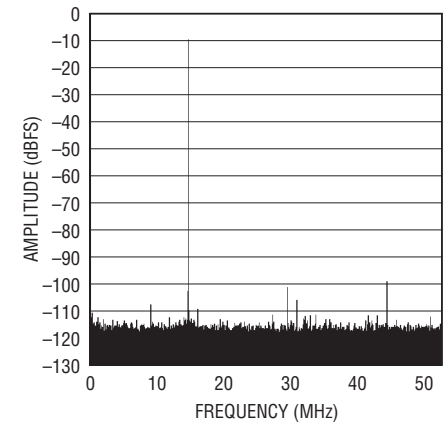
LTC2207: 64K Point FFT, f_{IN} = 14.8\text{MHz} , -10dBFS, PGA = 0, 105Msps
