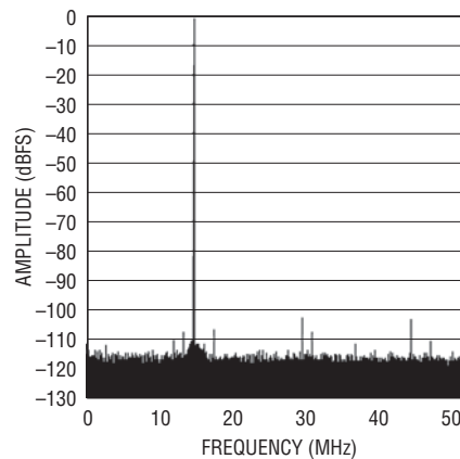
LTC2207: 64K Point FFT, f_{IN} = 14.8\text{MHz} , -1dBFS, PGA = 0, 105Msps
