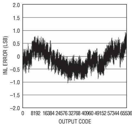
LTC2207: INL, 105Msps
