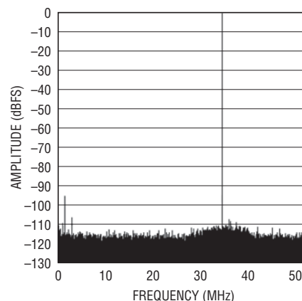
LTC2207: 64K Point FFT, f_{IN} = 140.2\text{MHz} , -1\text{dBFS} , \text{PGA} = 1 , 105Msps
