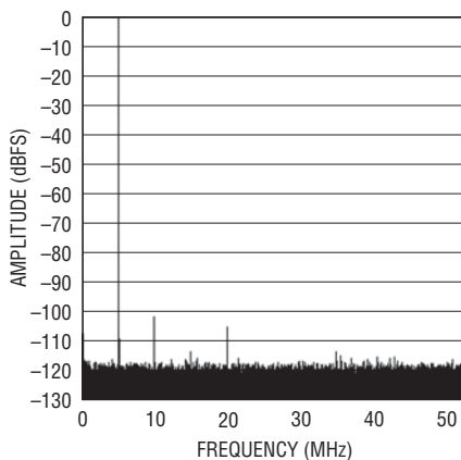
LTC2207: 128K Point FFT, f_{IN} = 4.93\text{MHz} , -1dBFS, PGA = 0, 105Msps
