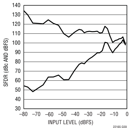
LTC2215 SFDR vs Input Level, f_{IN} = 70.5\text{MHz} , Dither "Off"
