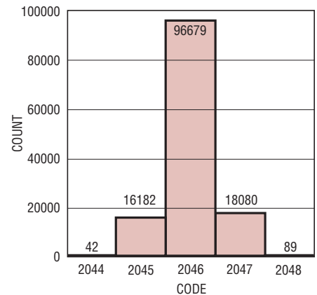
LTC2223: Shorted Input Noise Histogram
