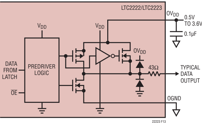
Figure 13. Digital Output Buffer
