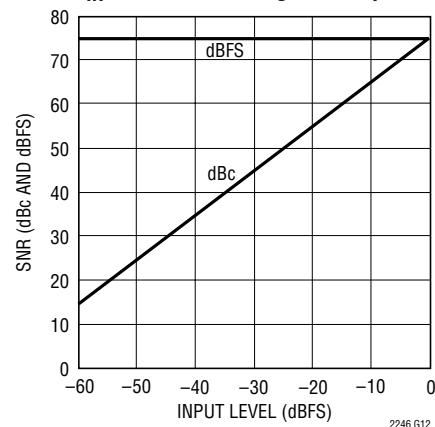
LTC2246: SNR vs Input Level, f_{IN} = 5\text{MHz} , 2V Range, 25Mpsps
