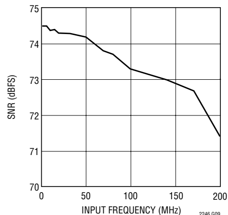
LTC2246: SNR vs Input Frequency, -1dB, 2V Range, 25Mpsps
