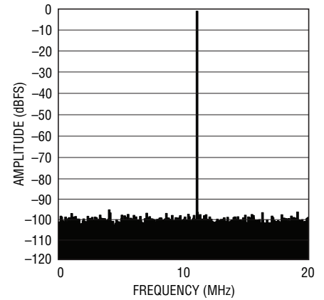
LTC2257-12: 8k Point FFT, f_{IN} = 29\text{MHz} , -1dBFS, 40Mps
