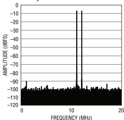
LTC2264-12: 8k Point 2-Tone FFT, f_{IN} = 68\text{MHz} , 69\text{MHz} , -1\text{dBFS} , 40Msps
