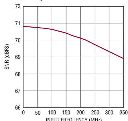
LTC2264-12: SNR vs Input Frequency, -1\text{dBFS} , 2V Range, 40Msps
