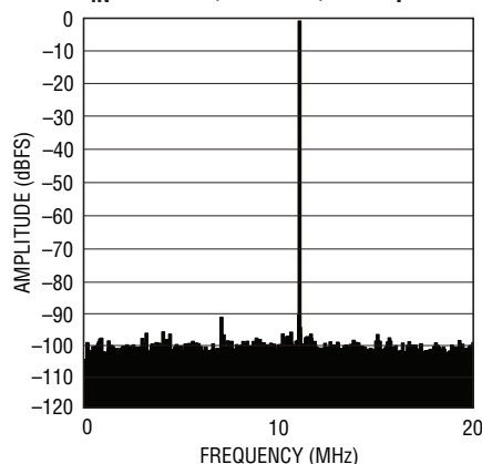
LTC2264-12: 8k Point FFT, f_{IN} = 69\text{MHz} , -1\text{dBFS} , 40Msps
