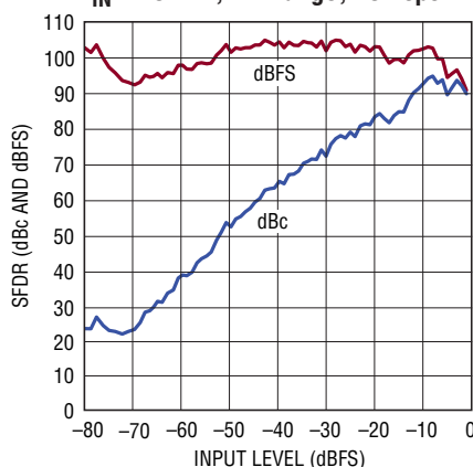
LTC2264-12: SFDR vs Input Level, f_{IN} = 70\text{MHz} , 2V Range, 40Msps
