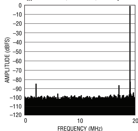
LTC2264-12: 8k Point FFT, f_{IN} = 139\text{MHz} , -1\text{dBFS} , 40Msps
