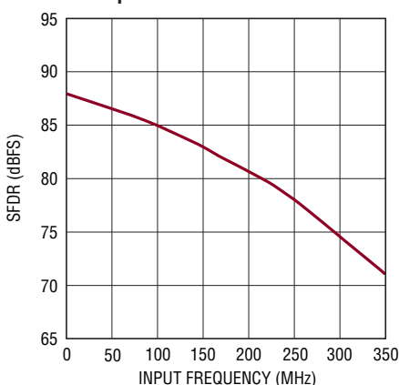
LTC2264-12: SFDR vs Input Frequency, -1\text{dBFS} , 2V Range, 40Msps
