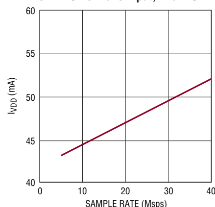
LTC2264-12: I_{VDD} vs Sample Rate, 5MHz Sine Wave Input, -1\text{dBFS}
