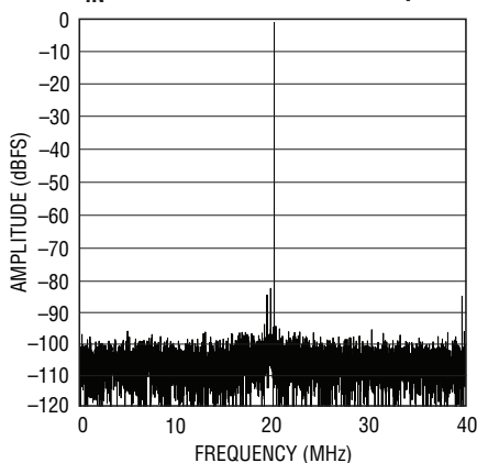
LTC2266-12: 8k Point FFT, f_{IN} = 140\text{MHz} , -1\text{dBFS} , 80\text{Mpsps}
