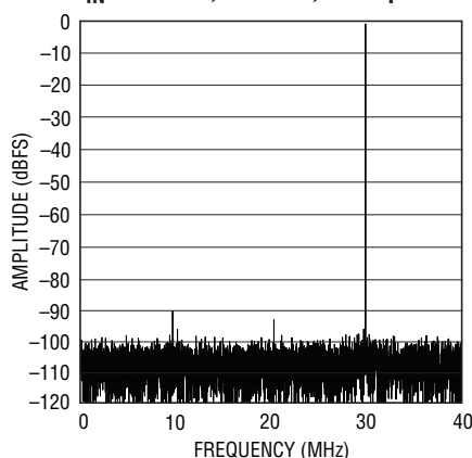
LTC2266-12: 8k Point FFT, f_{IN} = 30\text{MHz} , -1\text{dBFS} , 80\text{Mpsps}
