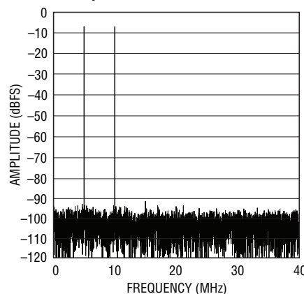
LTC2266-12: 8k Point 2-Tone FFT, f_{IN} = 70\text{MHz} , 75\text{MHz} , -1\text{dBFS} , 80\text{Mpsps}
