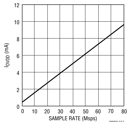
LTC2293: I_{OVPD} vs Sample Rate, 5MHz Sine Wave Input, -1dB, O_{VDD} = 1.8\text{V}
