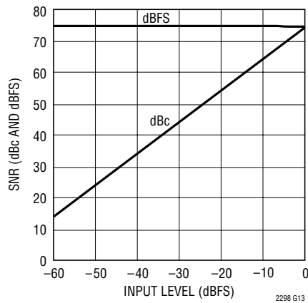
LTC2298: SNR vs Input Level, f_{IN} = 30\text{MHz} , 2V Range, 65Mps
