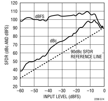
LTC2298: SFDR vs Input Level, f_{IN} = 30\text{MHz} , 2V Range, 65Mps
