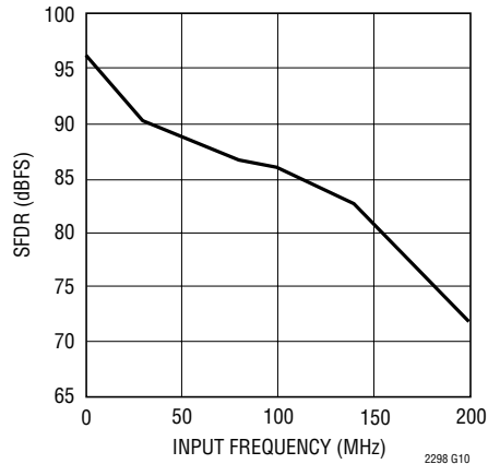
LTC2298: SFDR vs Input Frequency, -1dB, 2V Range, 65Mps
