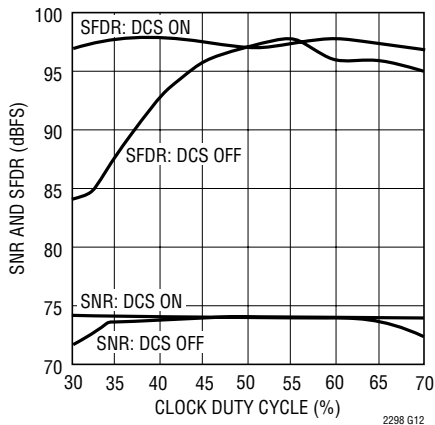
LTC2298: SNR and SFDR vs Clock Duty Cycle, 65Mps
