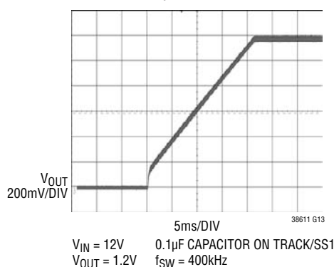
Soft-Start Start-Up Response (2-Phase Using D12S1R845A Power Block)
