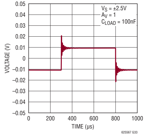
Small-Signal Response
