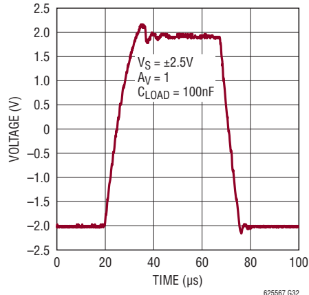
Large-Signal Response
