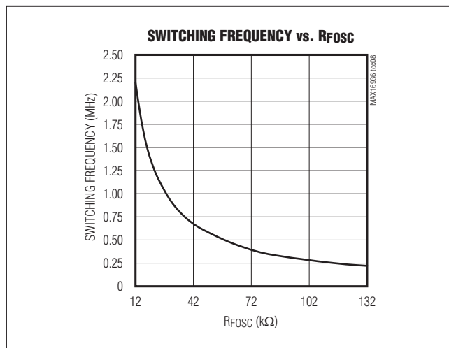
Figure 3. Switching Frequency vs. Rfosc (see Figure 3).
