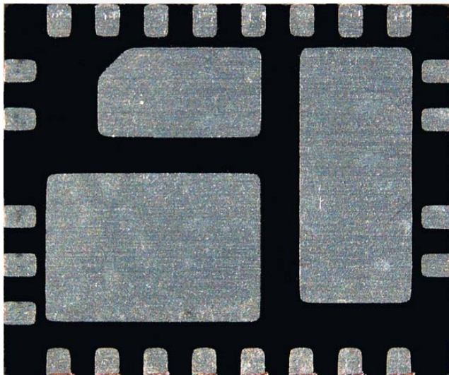
Figure 1: Bottom side view showing pads for TinyBuck™
