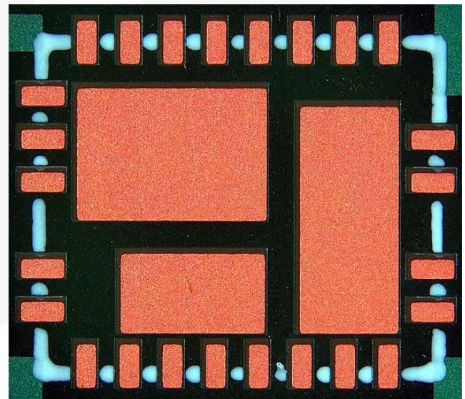
Figure 3: PWB pad showing OSP pad finish.
