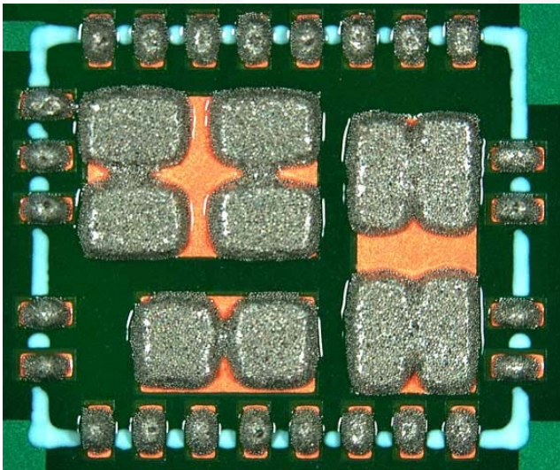
Figure 4: Printed Solder Paste.
