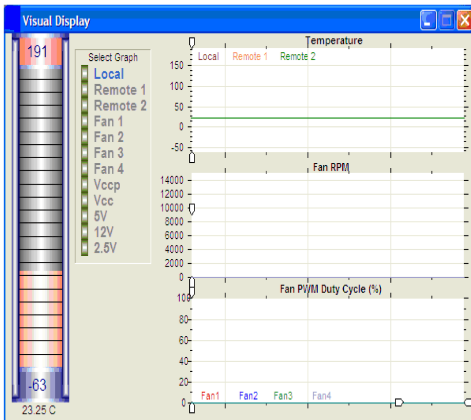
Figure 5. Graphing Window
