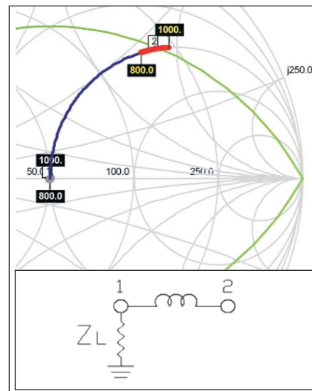
Figure 8 · Z_0 = 50 , Q = 1.75 ; N1-2 Series L = 15nH.
