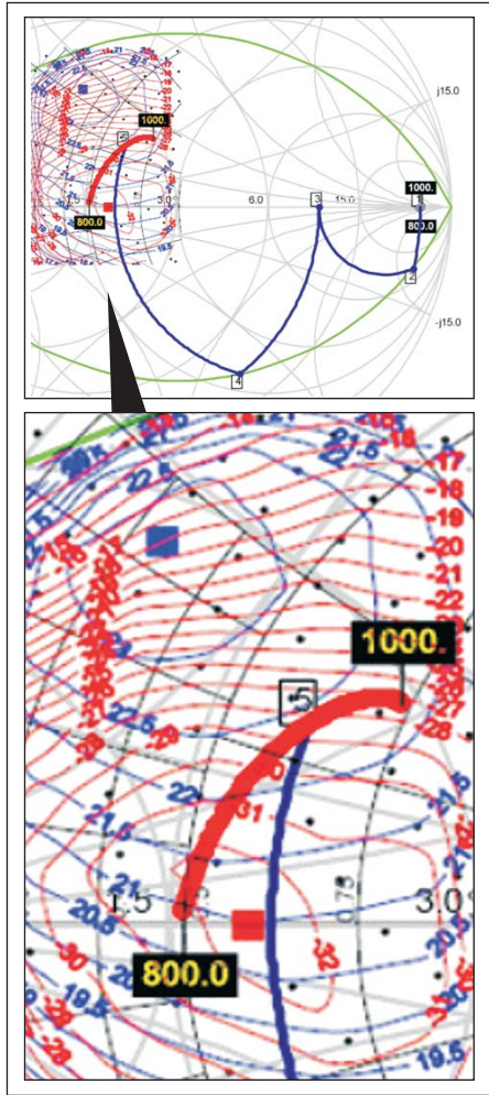
Figure 5 · Trajectory relative to 60W PEP LDMOS Load Pull contours (19): Z_O = 3 , 28V DC , 900 MHz; Max Gain = 23.6 dB @ Z = 1.0 + j1.3 ; Min IMD3 = -32.7 dBc @ Z = 1.0 + j0.0 ; Max Eff = 66.75% @ Z = 0.9 + j1.8 .
