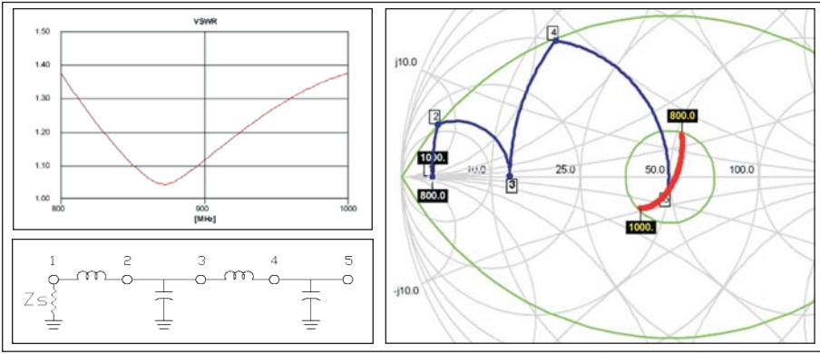
Figure 4 · Z_O = 50 , Z_S = 3 , Q = 1.75 , SWR = 1.4 ; N1-2 Series L = 0.9 pH, N2-3 Shunt C = 25 pF; N3-4 Series L = 3.8 nH, N4-5 Shunt C = 6.5 pF.
