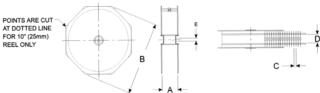
Lead-Tape Specifications: Reeled in accordance with EIA-296-F
