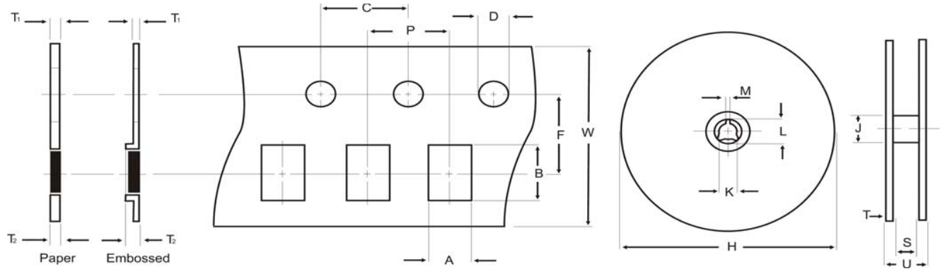
RACF16 - RACF64 Packaging Specifications
