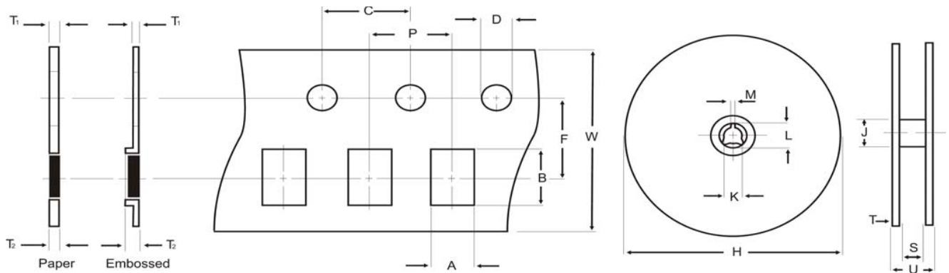
RAVF10 - RAVF32 Packaging Specifications
