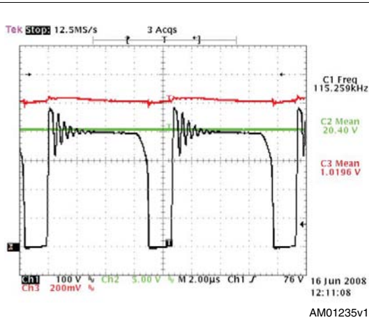
Figure 5. V_{IN} = 230\text{ V}_{AC} - 50\text{ Hz} , full load, normal operation
