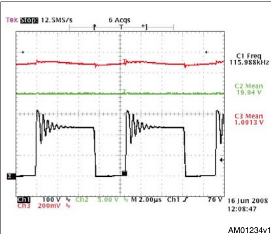
Figure 4. V_{IN} = 115\text{ V}_{AC} - 60\text{ Hz} , full load, normal operation
