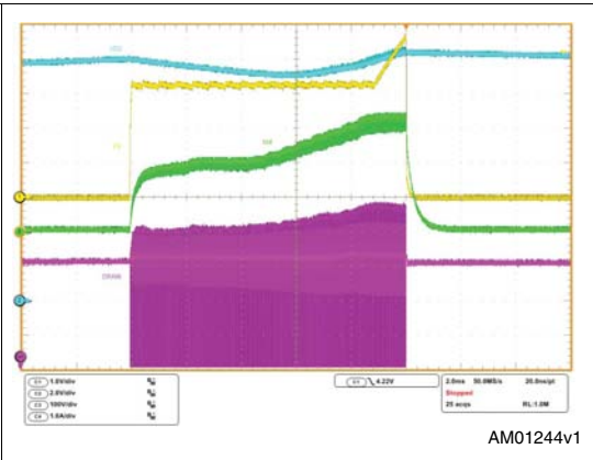
Figure 14. V_{IN} = 230\text{ V}_{AC} - 50 Hz short-circuit operation detail
