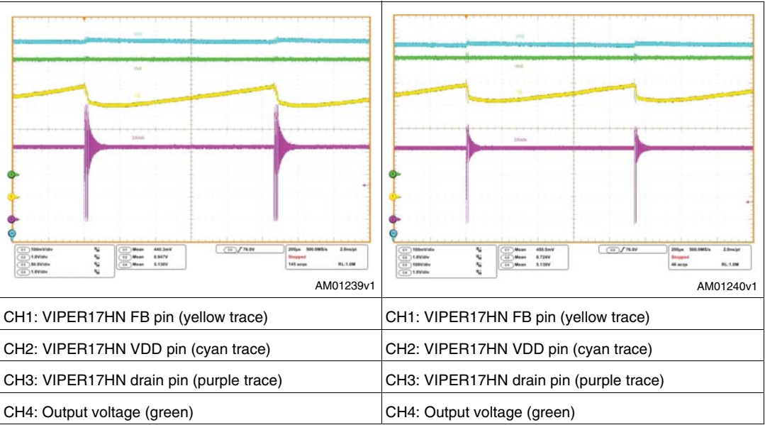
Figure 9. V_{IN} = 115\text{ V}_{AC} - 50\text{ Hz} in no-load condition
