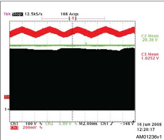
Figure 6. V_{IN} = 230\text{ V}_{AC} - 50\text{ Hz} , full load, FB pin behavior
