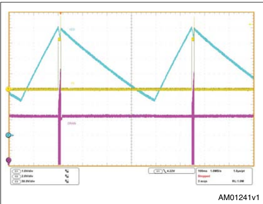
Figure 11. V IN = 115 V AC - 60 Hz short-circuit operation
