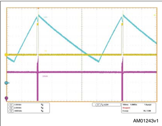
Figure 13. V_{IN} = 115\text{ V}_{AC} - 60 Hz short-circuit operation
