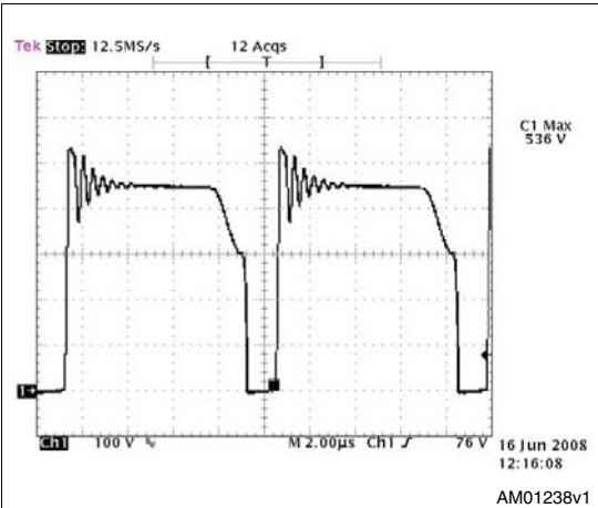
Figure 8. V_{IN} = 265\text{ V}_{AC} - 50\text{ Hz} , full load, maximum drain peak voltage
