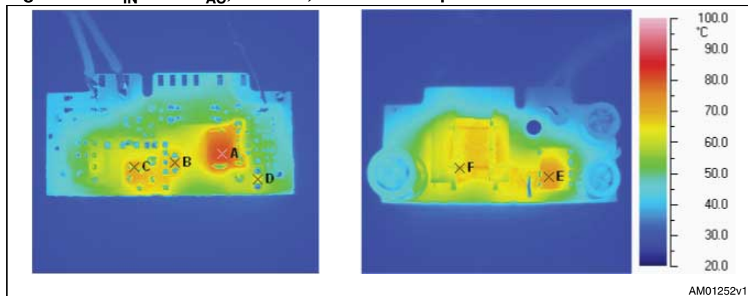
Figure 22. V_{IN} = 230\text{ V}_{AC} , full load, bottom and top sides
