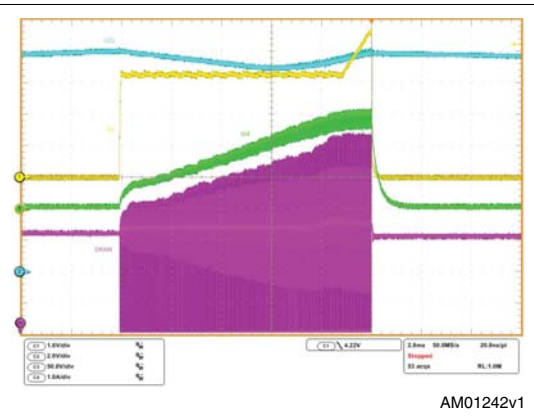
Figure 12. V IN = 230 V AC - 50 Hz short-circuit operation detail
