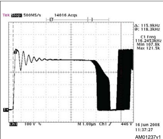
Figure 7. V_{IN} = 230\text{ V}_{AC} - 50\text{ Hz} , full load, frequency modulation
