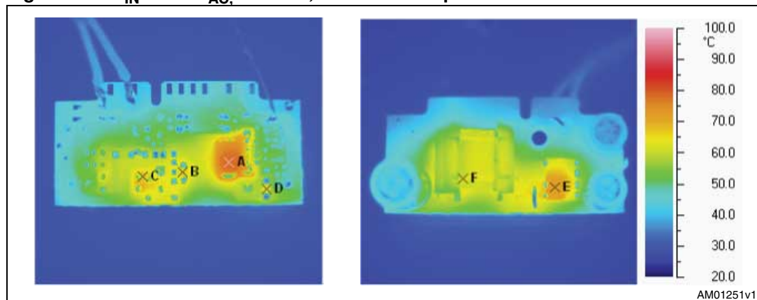
Figure 21. V_{IN} = 115\text{ V}_{AC} , full load, bottom and top sides
