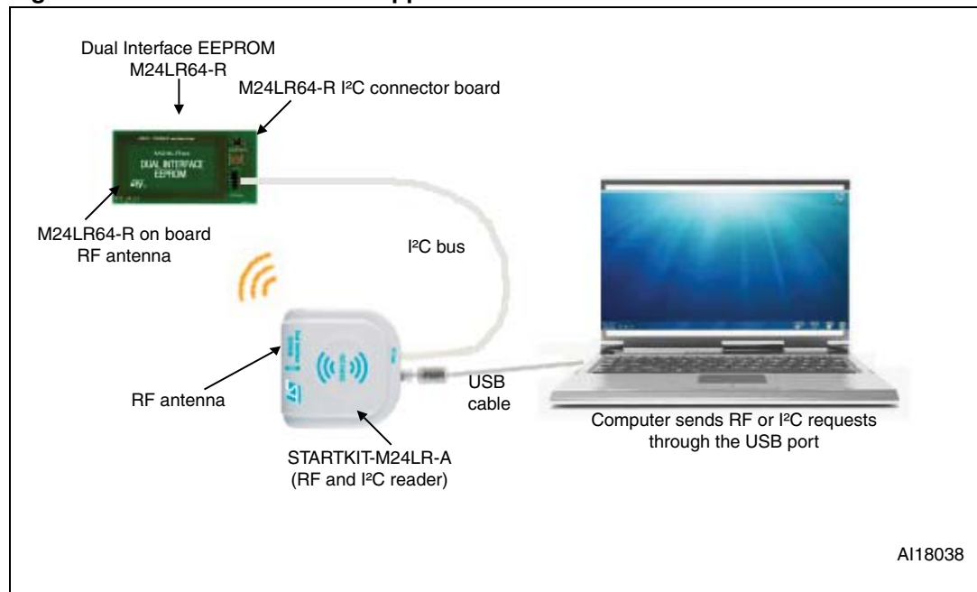
Figure 2. STARTKIT-M24LR-A application schematics
