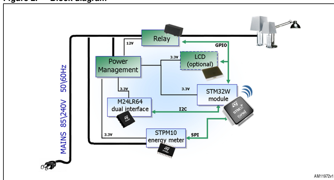
Figure 2. Block diagram
