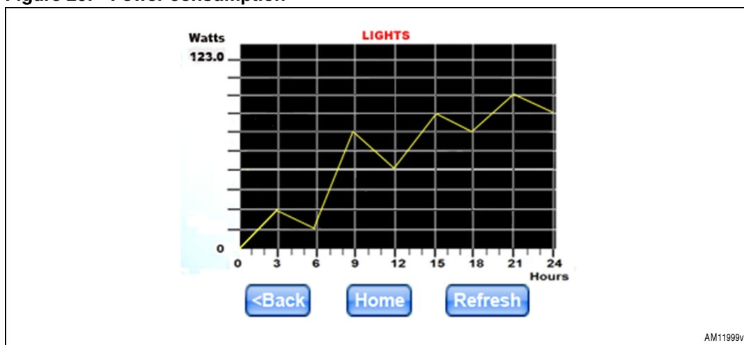
Figure 29. Power consumption
