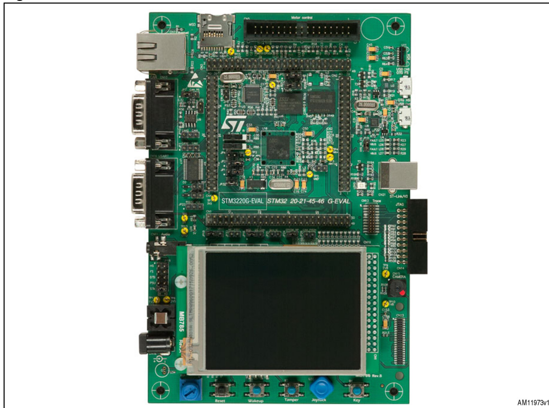
Figure 3. STM3220G-EVAL board
