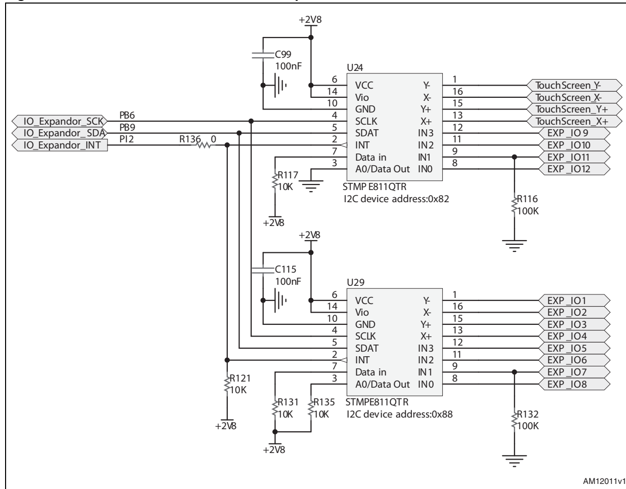
Figure 46. STM3220-21-45-46G-EVAL I/O_Expander
