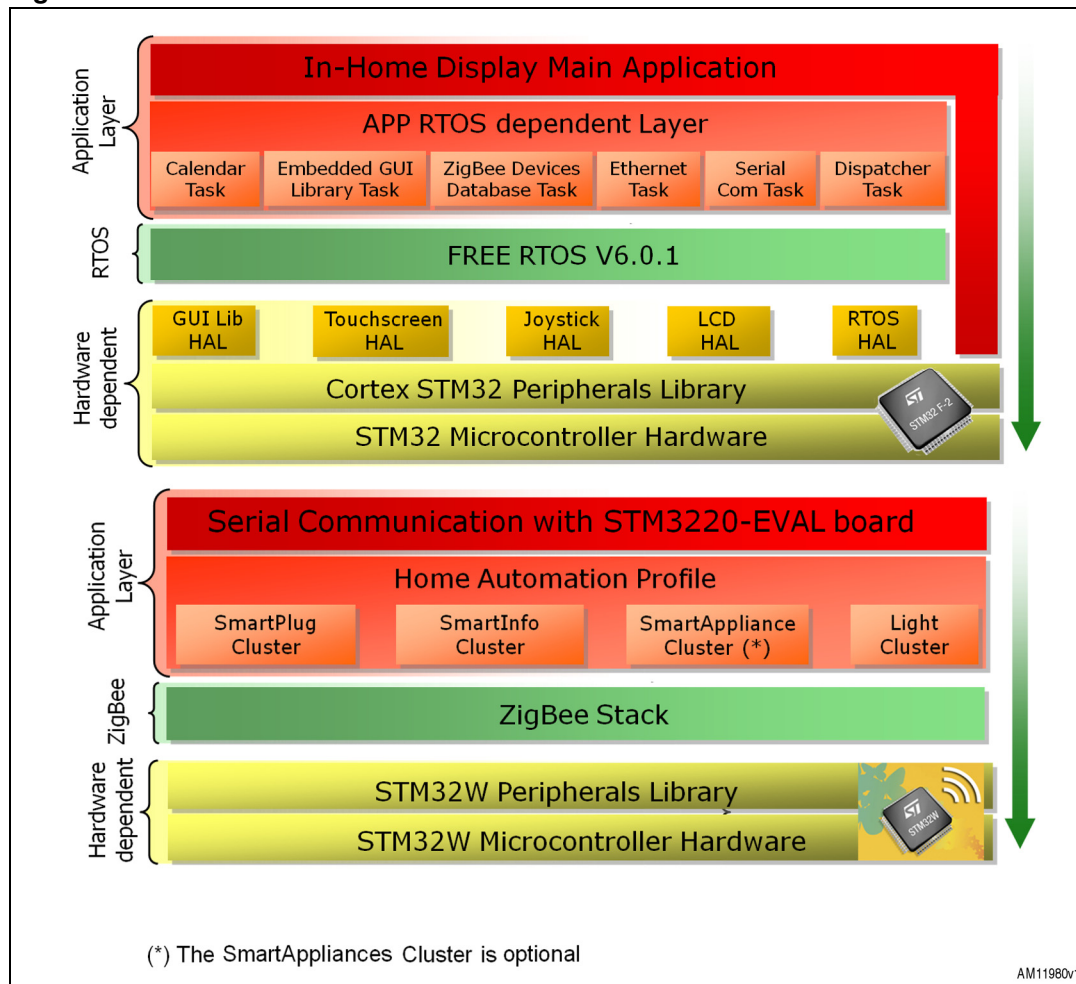
Figure 10. Firmware architecture
