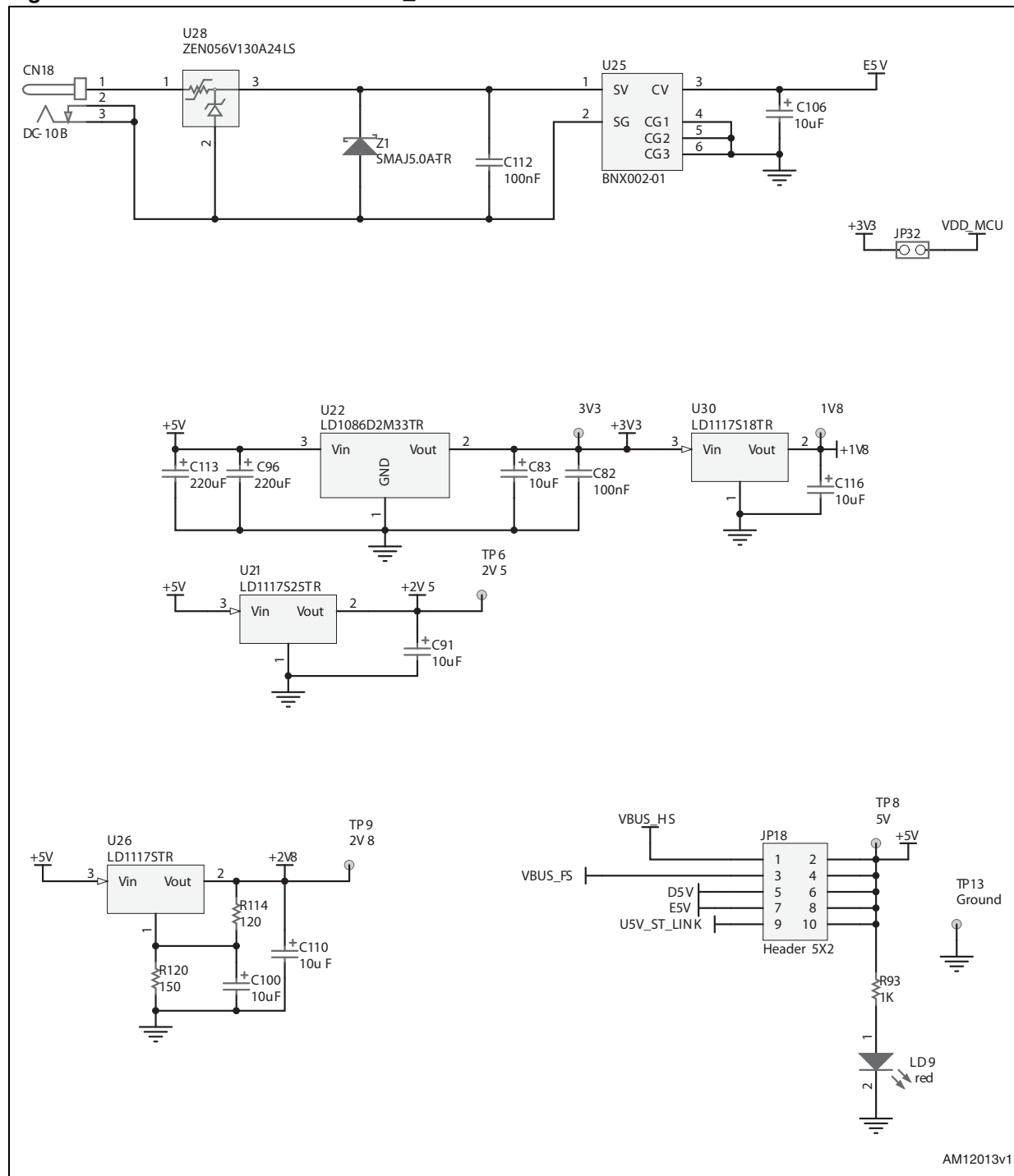
Figure 48. STM3220-21-45-46G-EVAL_Power
