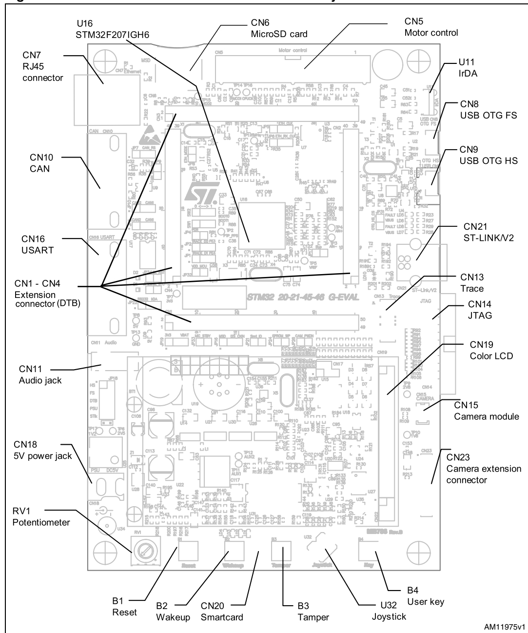
Figure 5. STM3220G-EVAL demonstration board layout
