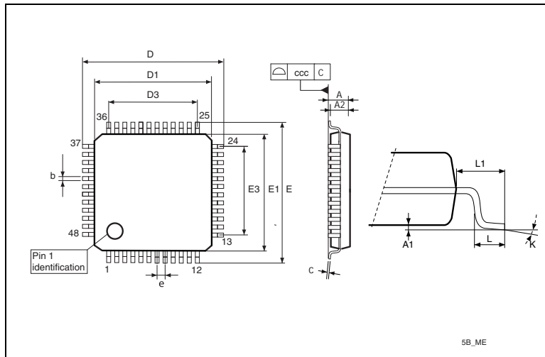
Figure 9. LQFP48 – 7 x 7mm, 48-pin low-profile quad flat package outline (1)
