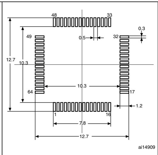
Figure 8. Recommended footprint (1)(2)
