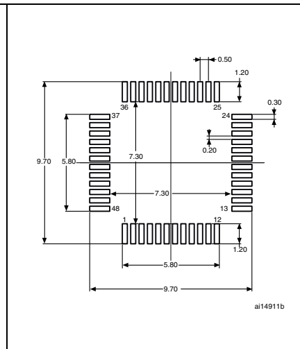
Figure 10. Recommended footprint (1)(2)
