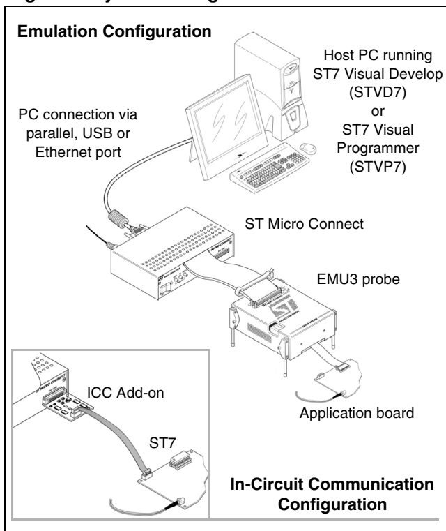
Figure 1: System configurations
