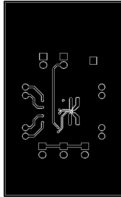
Figure 5. PCB bottom layer
