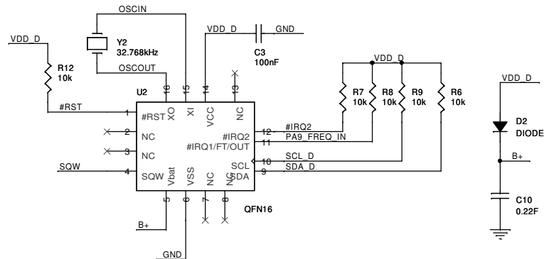
M41T83S_QFN
