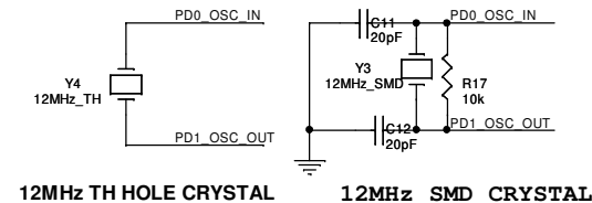
12MHz TH HOLE CRYSTAL
