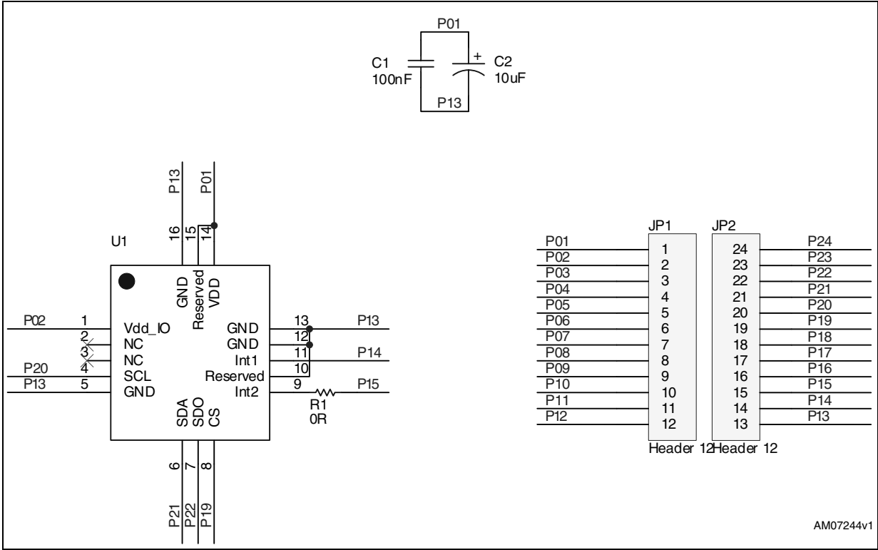
Figure 1. STEVAL-MKI091V1 adapter board circuit schematic
