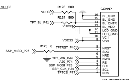
MB542 TFT CONNECTOR
