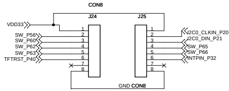
KEY BOARD CONNECTOR
