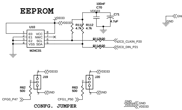
CONFIG. JUMPER
