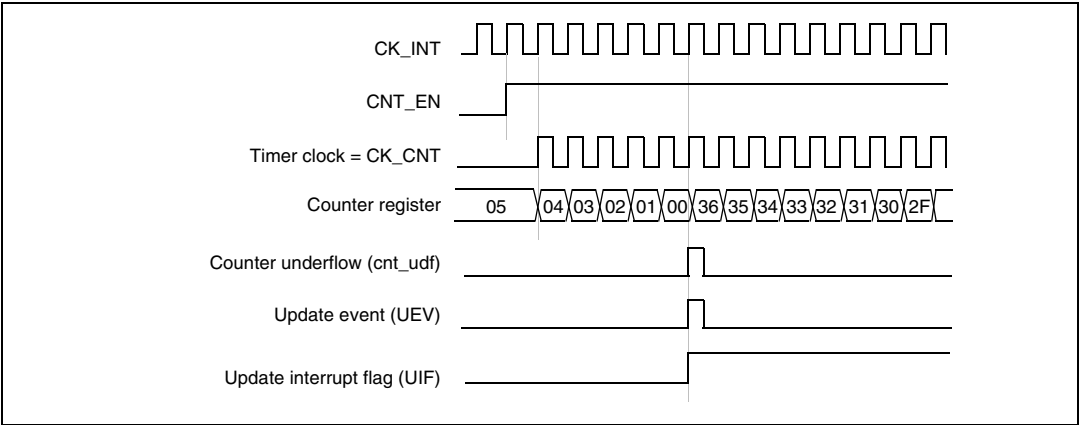
Figure 109. Counter timing diagram, internal clock divided by 1
