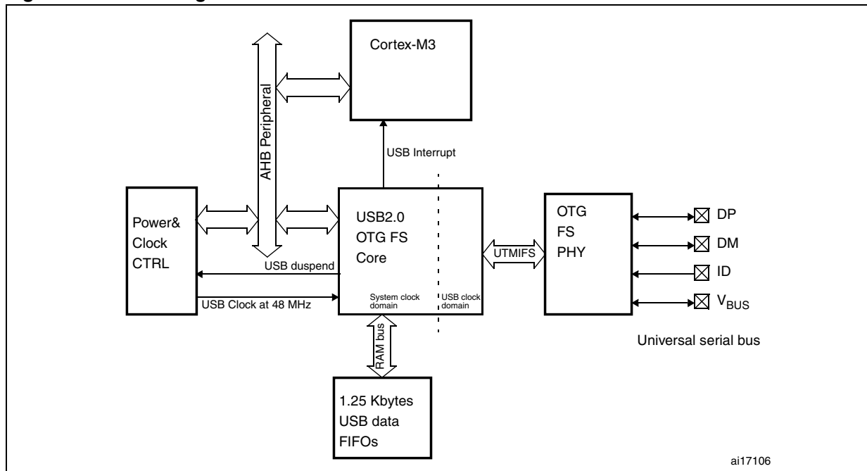
Figure 301. Block diagram
