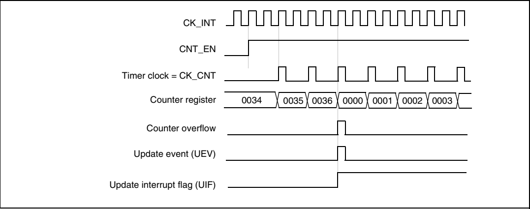
Figure 173. Counter timing diagram, internal clock divided by 2
