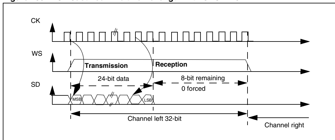
Figure 255. MSB Justified 24-bit frame length with CPOL = 0
