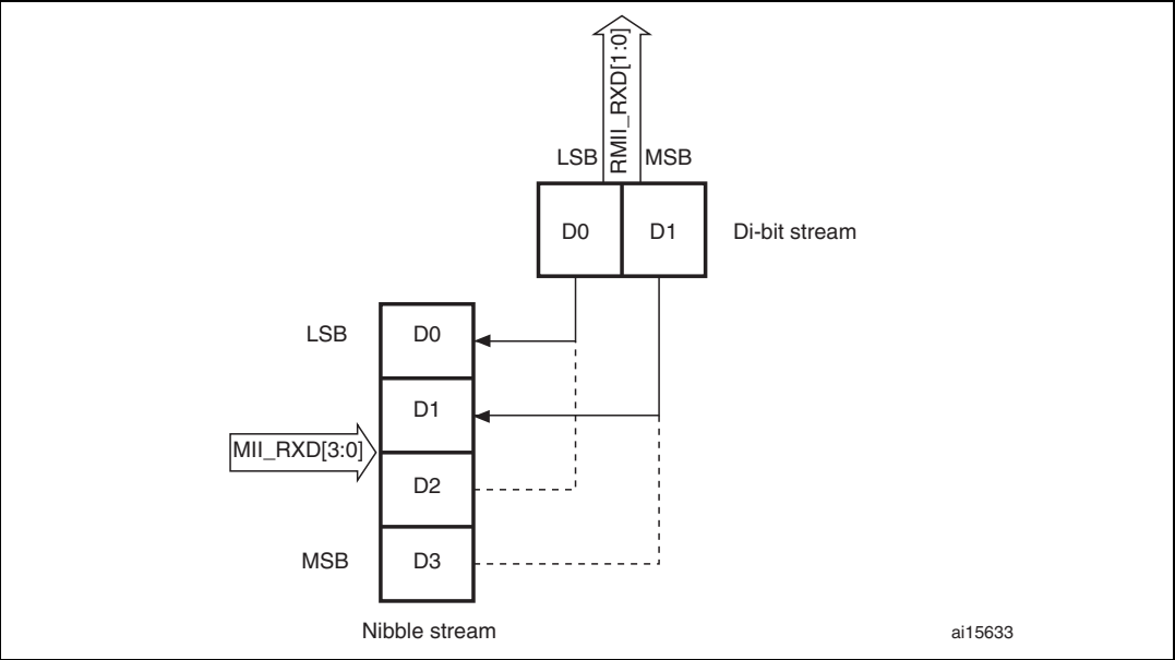
Figure 341. Receive bit order
