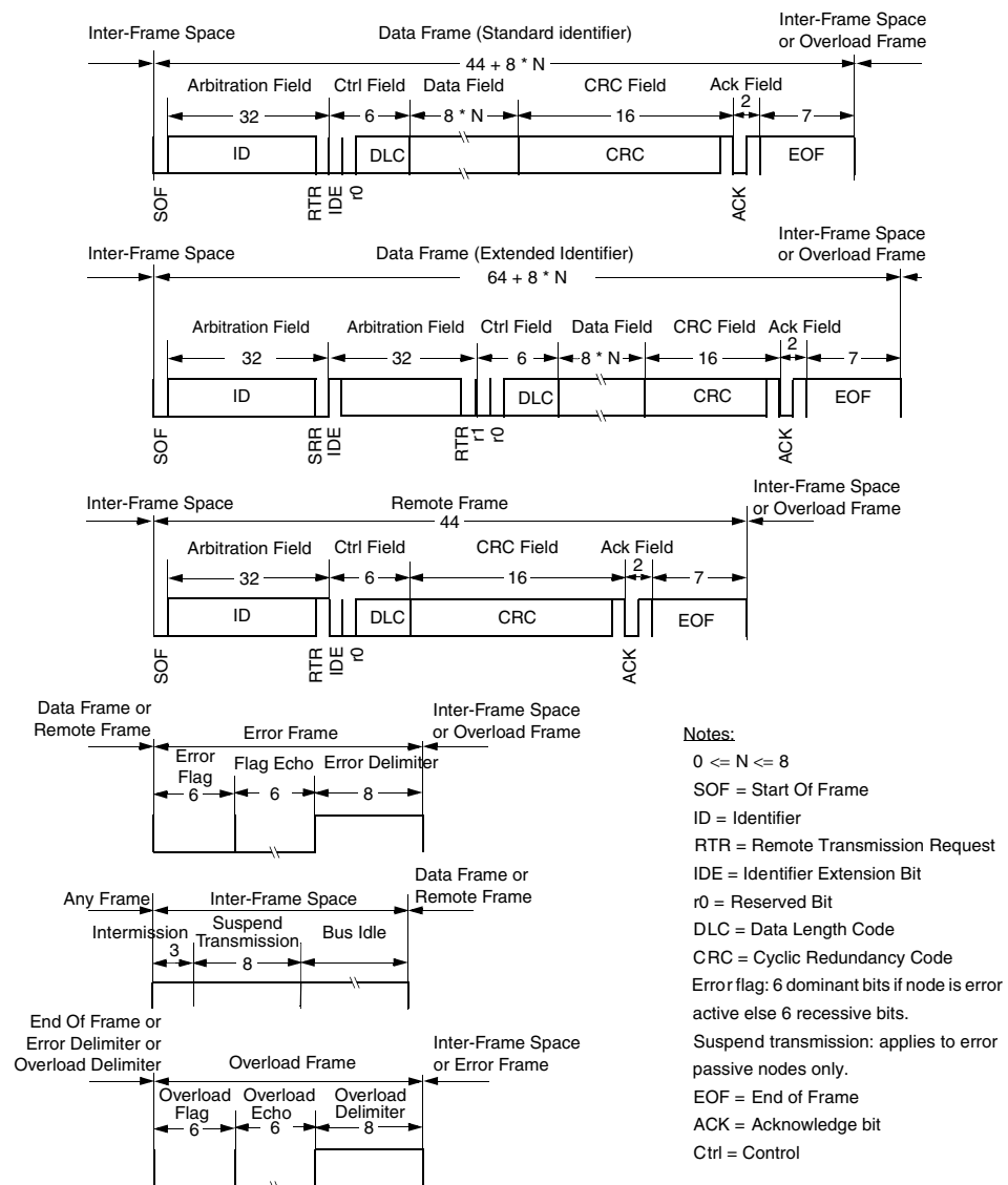
Figure 234. CAN frames
