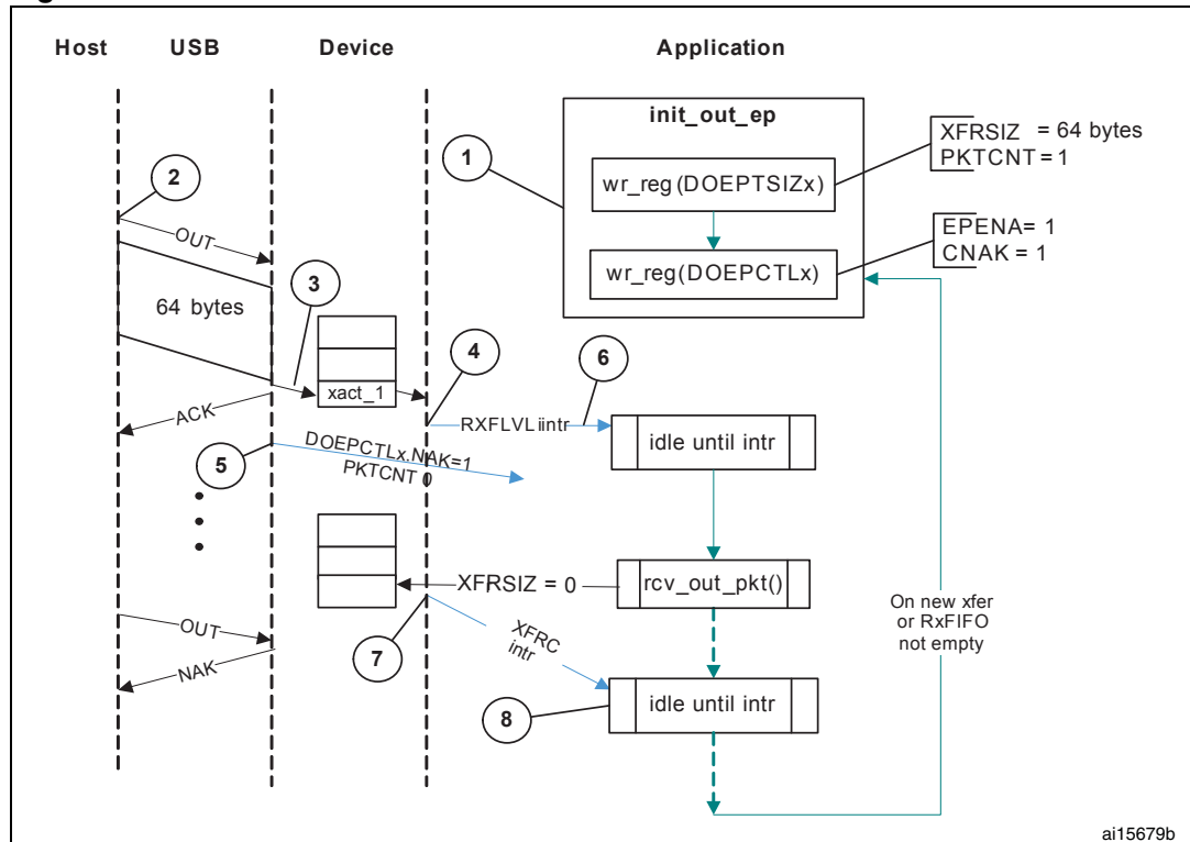
Figure 319. Bulk OUT transaction
