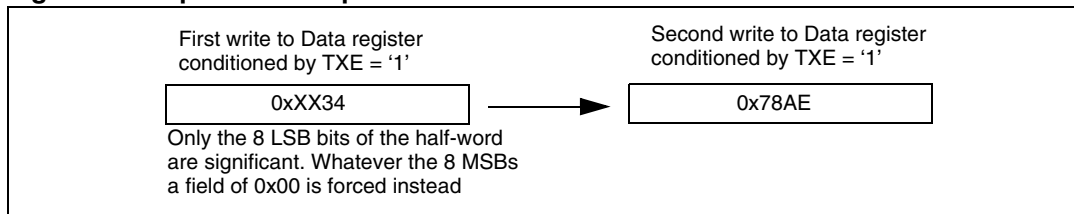
Figure 259. Operations required to transmit 0x3478AE
