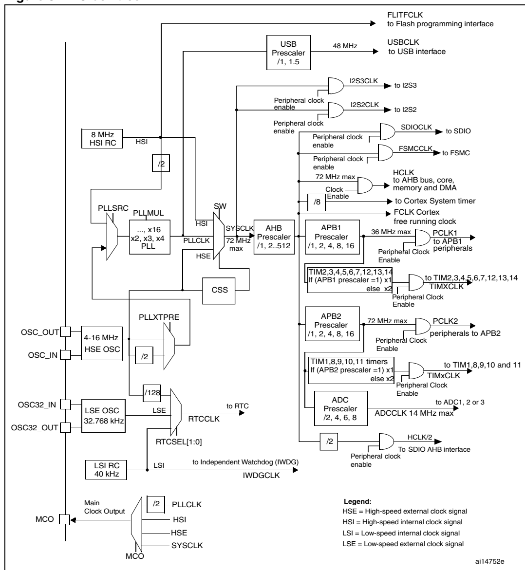
Figure 8. Clock tree
