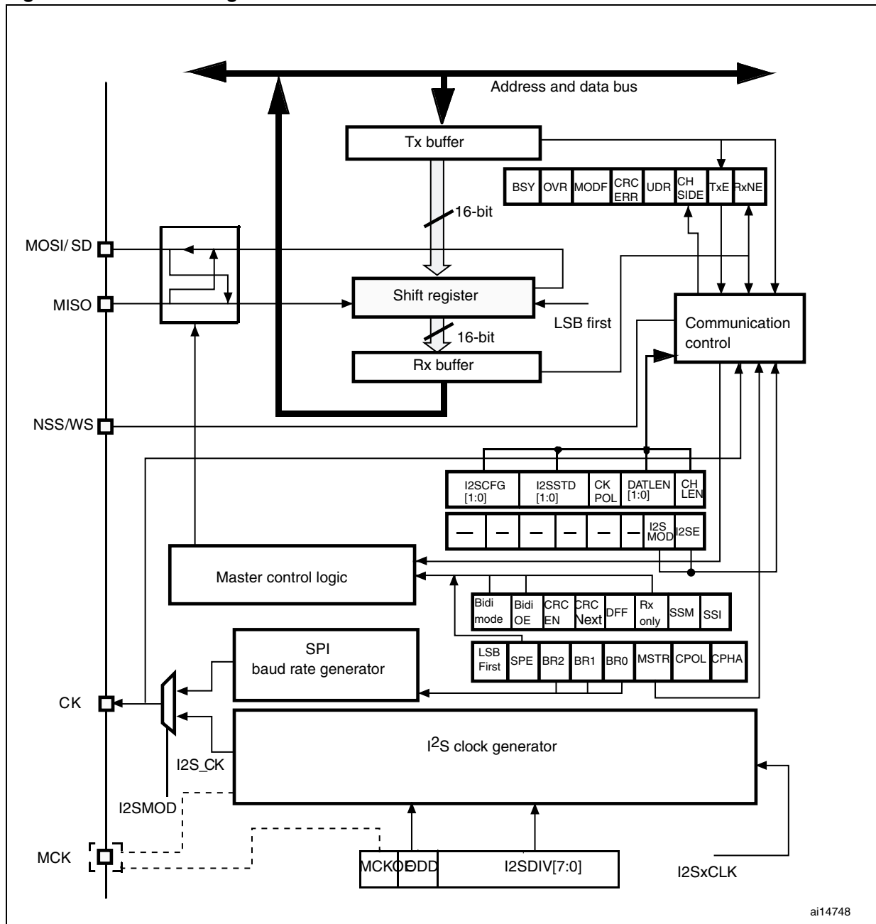
Figure 247. I 2 S block diagram
