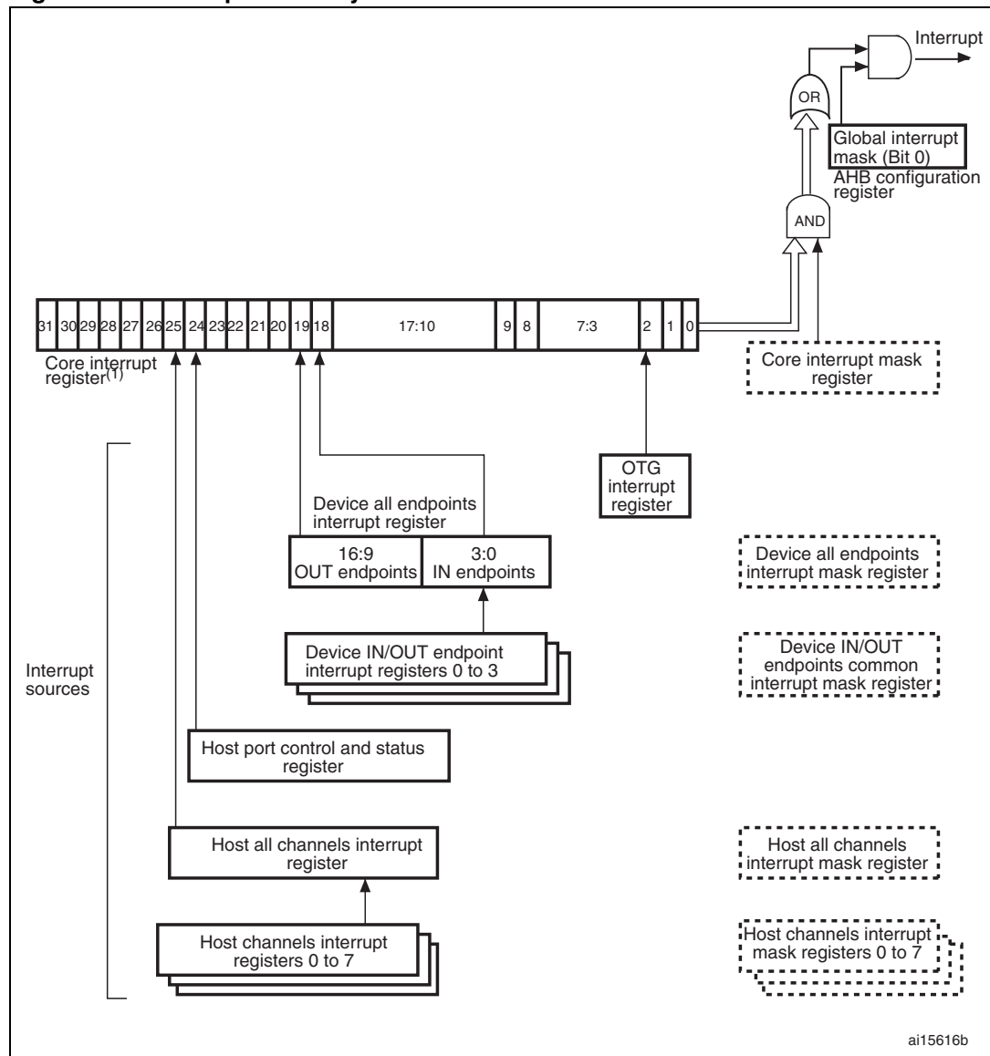
Figure 309. Interrupt hierarchy
