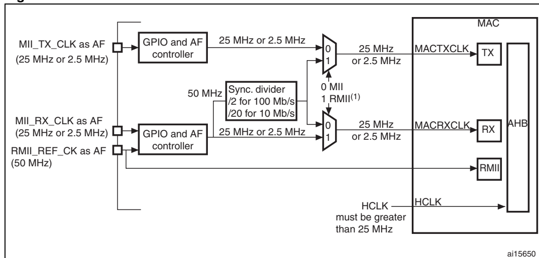
Figure 333. Clock scheme
