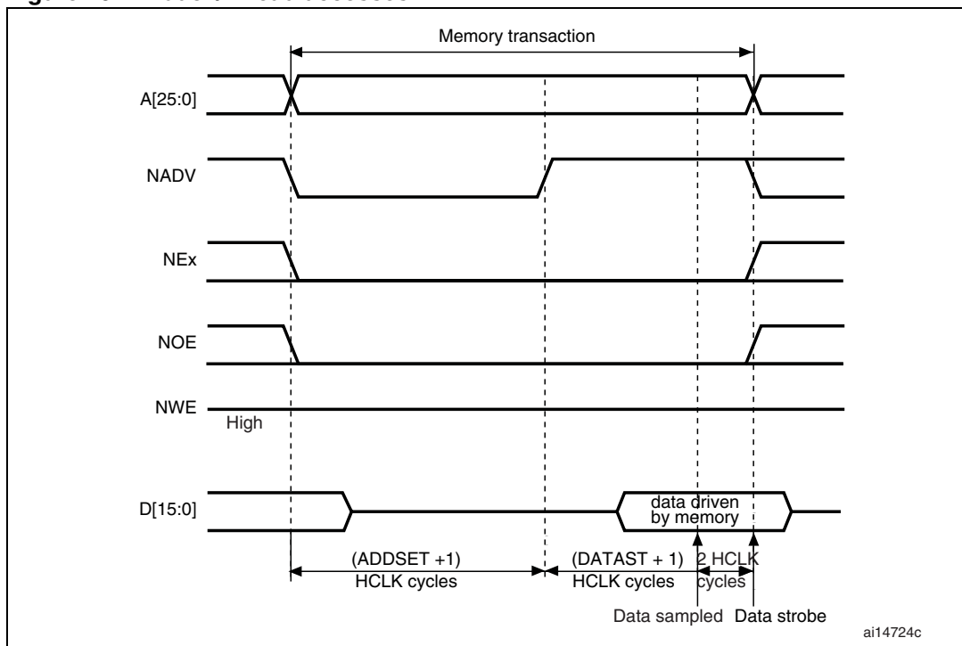
Figure 191. Mode2/B read accesses
