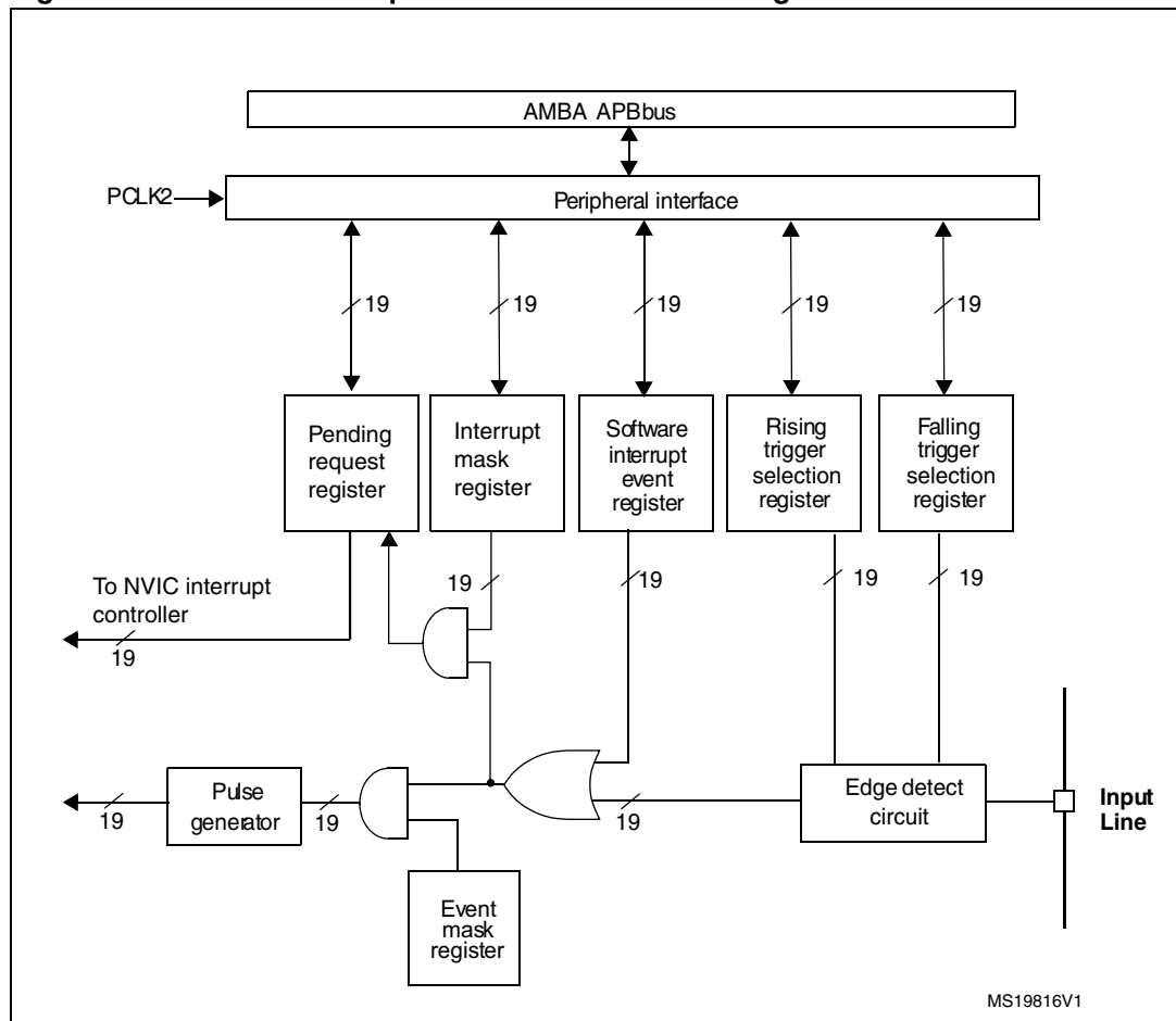
Figure 20. External interrupt/event controller block diagram
