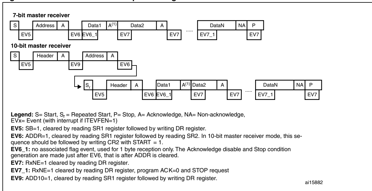
Figure 272. Method 1: transfer sequence diagram for master receiver
