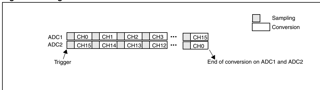
Figure 31. Regular simultaneous mode on 16 channels
