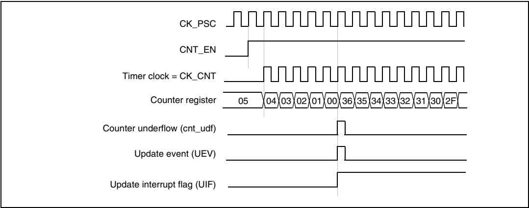
Figure 61. Counter timing diagram, internal clock divided by 1
