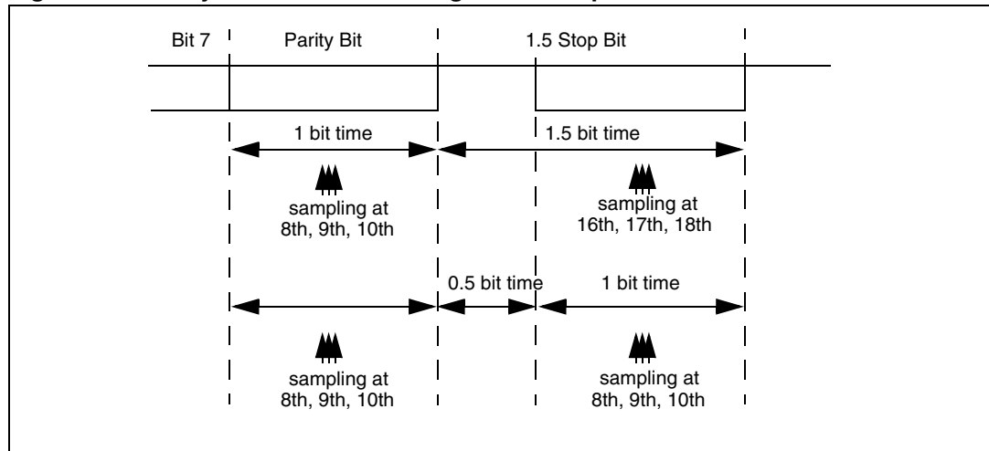
Figure 292. Parity error detection using the 1.5 stop bits
