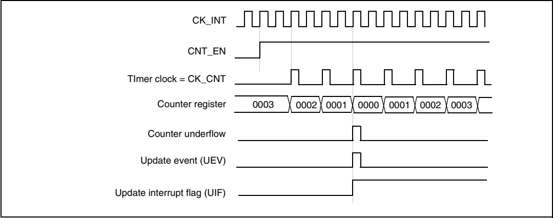
Figure 115. Counter timing diagram, internal clock divided by 2
