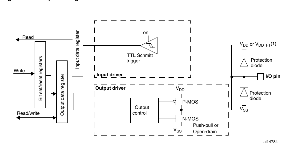
Figure 16. Output configuration
