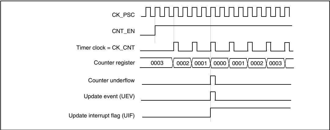
Figure 67. Counter timing diagram, internal clock divided by 2
