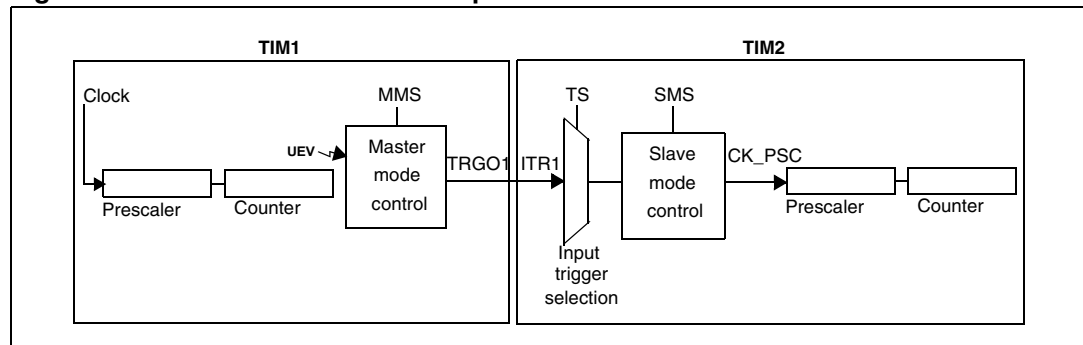
Figure 140. Master/Slave timer example
