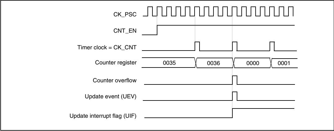
Figure 152. Counter timing diagram, internal clock divided by 4
