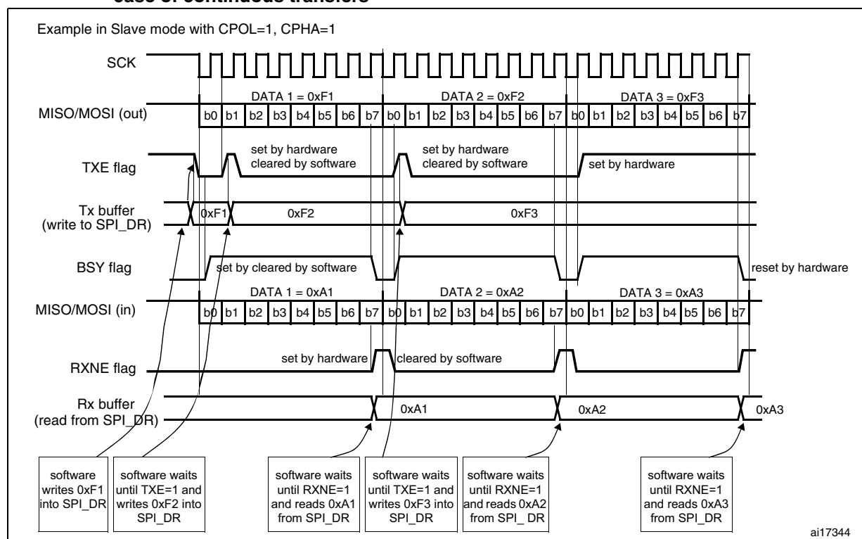
Figure 240. TXE/RXNE/BSY behavior in Slave / full-duplex mode (BIDIMODE=0, RXONLY=0) in the case of continuous transfers
