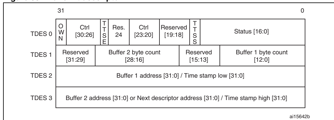
Figure 354. ransmit descriptor
