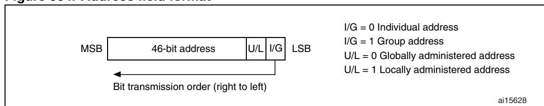
Figure 334. Address field format
