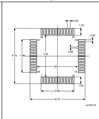
Figure 13. Recommended footprint (1)(2)
