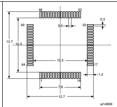
Figure 11. Recommended footprint (1)(2)
