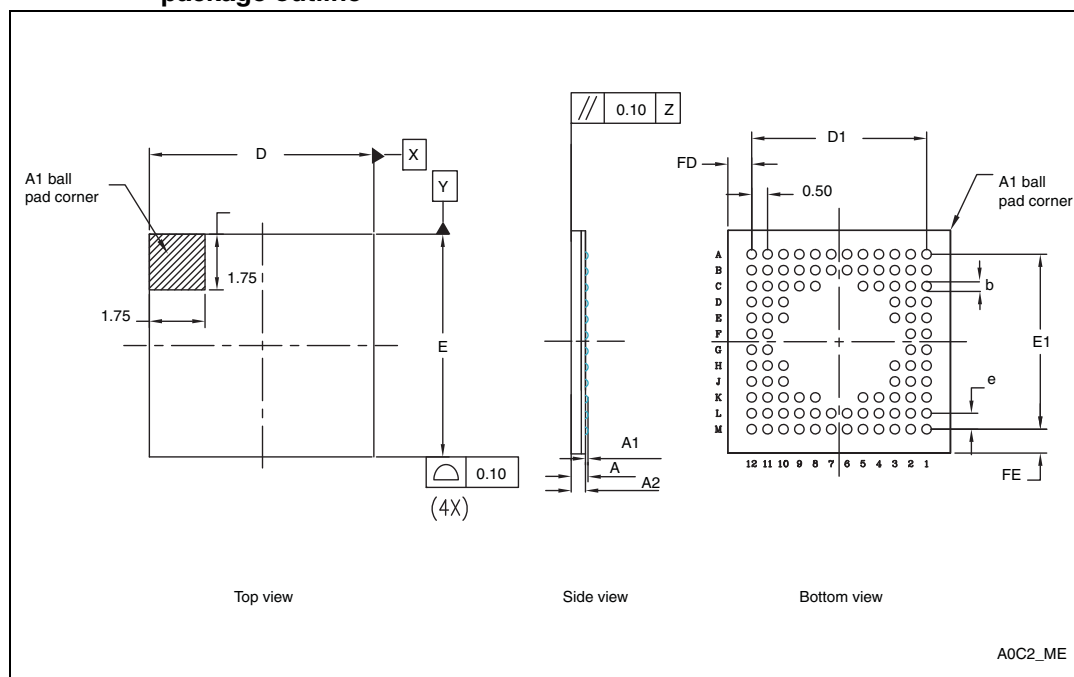
Figure 8. UFBGA100 – ultra fine pitch ball grid array, 7 x 7 mm, 0.50 mm pitch, package outline
