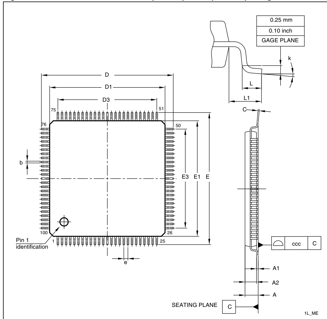
Figure 10. LQFP100 –14 x 14 mm 100-pin low-profile quad flat package outline
