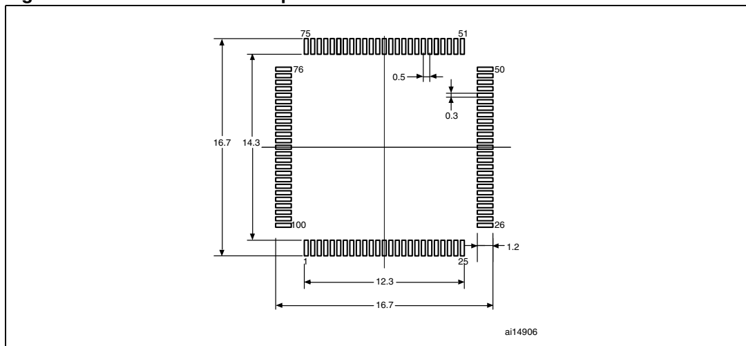
Figure 11. Recommended footprint
