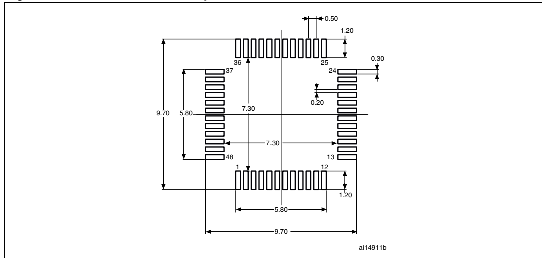
Figure 15. Recommended footprint
