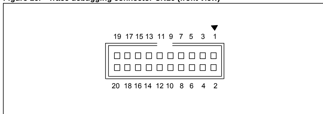
Figure 16. Trace debugging connector CN10 (front view)
