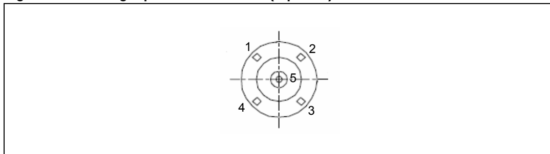
Figure 10. Analog input connector CN3 (top view)
