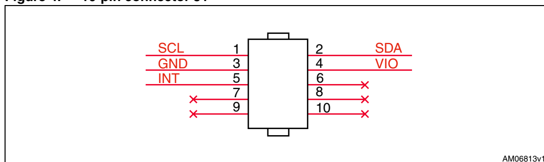
Figure 4. 10-pin connector J1
