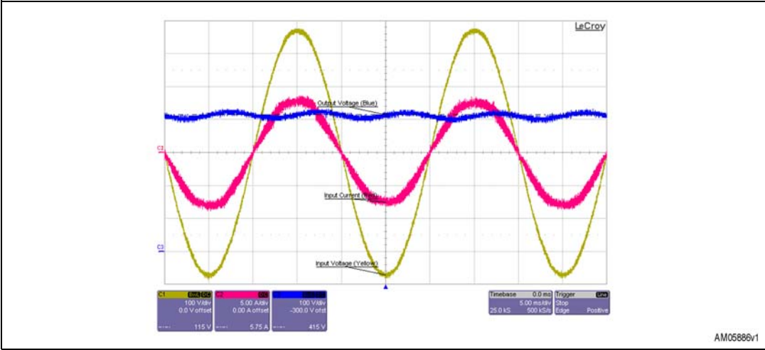
Figure 42. 265 Vrms at 50 Hz as input - 1400 W as output load
