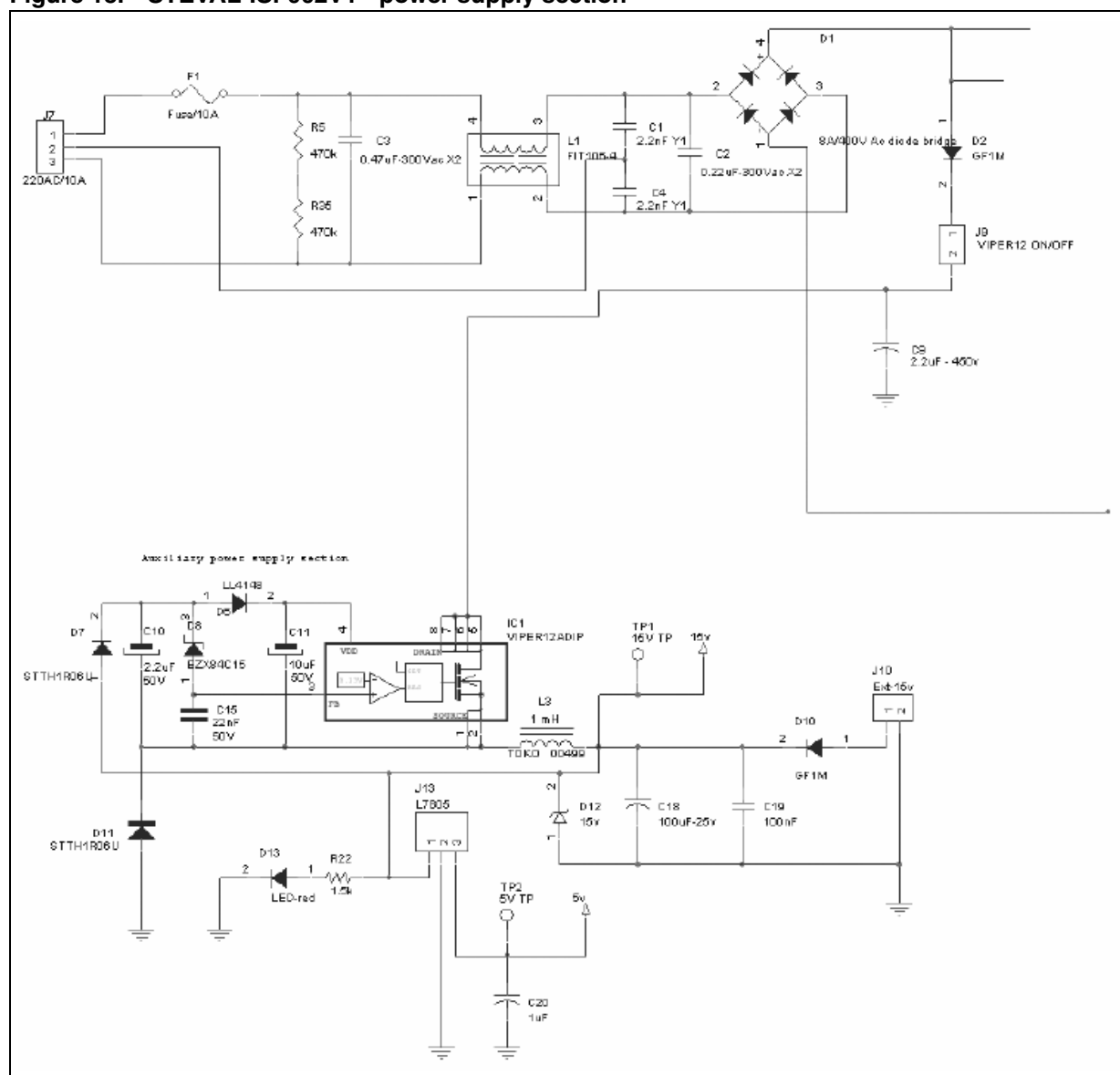
Figure 13. STEVAL-ISF002V1 - power supply section
