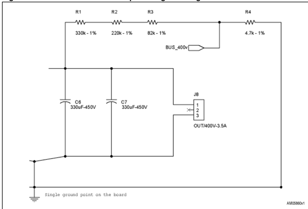
Figure 16. STEVAL-ISF002V1 - output voltage sensing section
