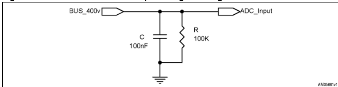
Figure 17. STEVAL-IHM022V1 - output voltage sensing section
