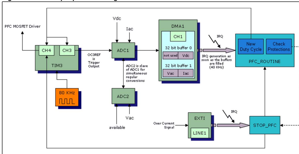
Figure 28. Use of peripherals for digital PFC
