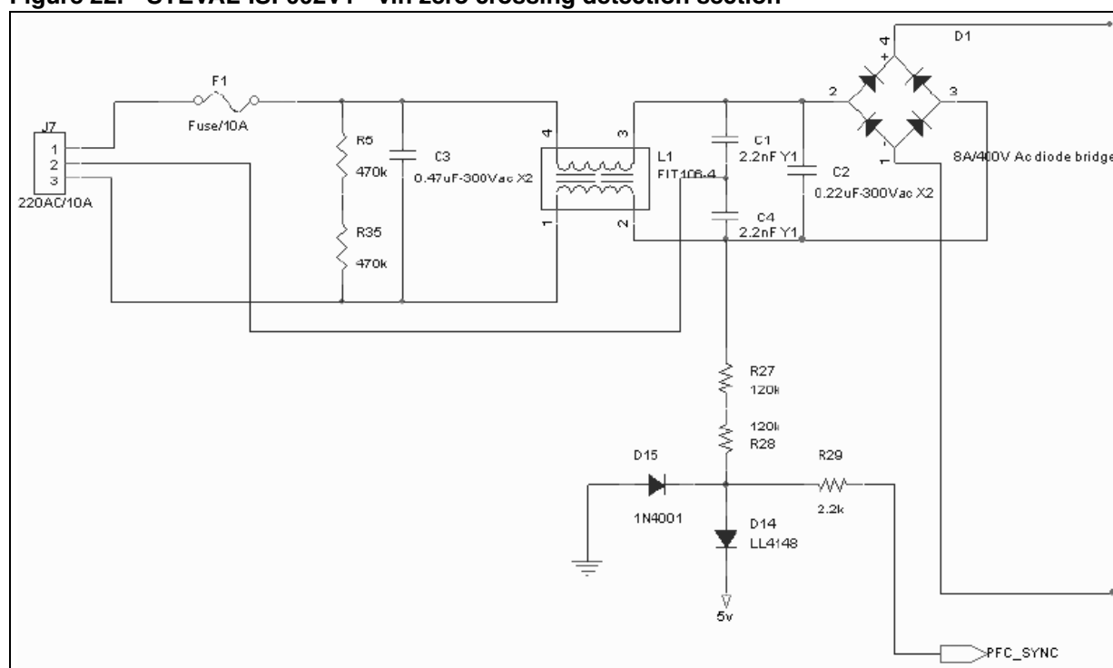
Figure 22. STEVAL-ISF002V1 - vin zero crossing detection section
