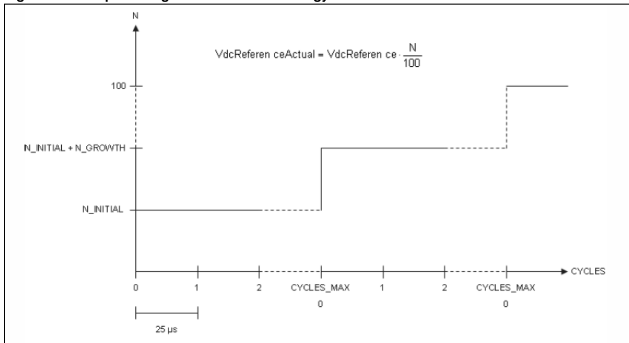
Figure 26. Output voltage soft-start methodology
