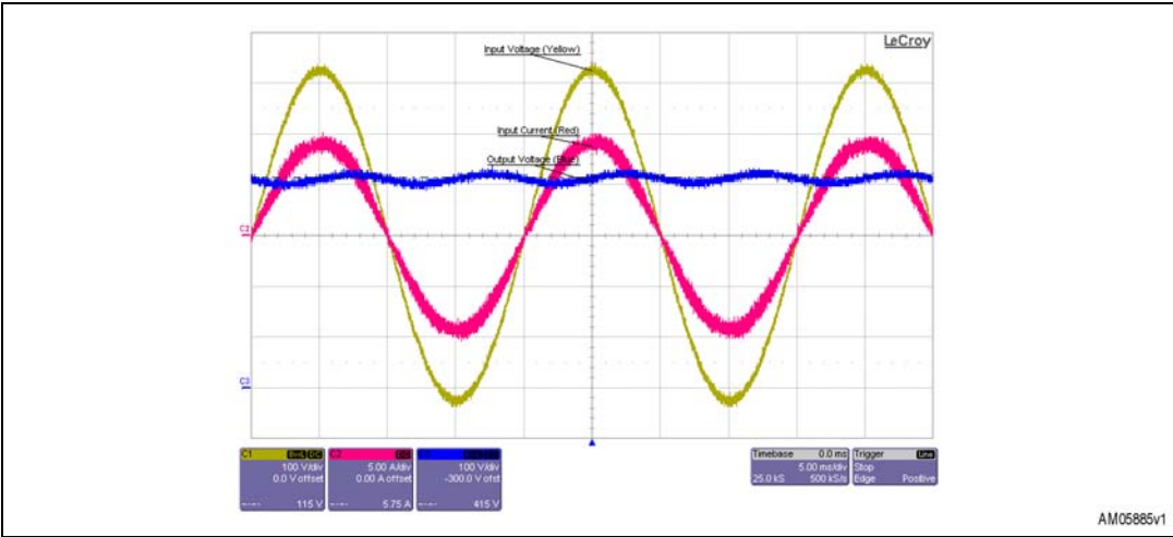
Figure 41. 230 Vrms at 50 Hz as input - 1400 W as output load
