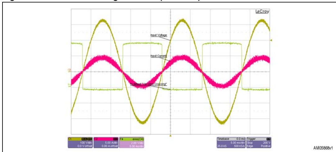
Figure 24. Vin zero crossing detection (with load)
