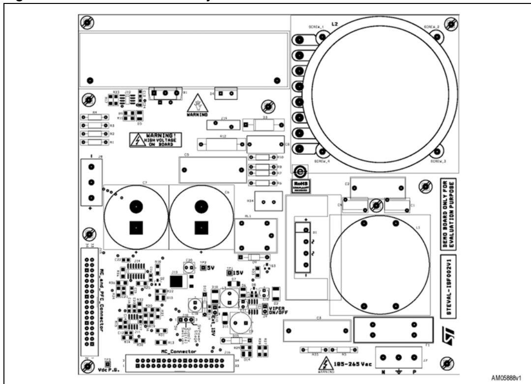
Figure 44. STEVAL-ISF002V1 layout
