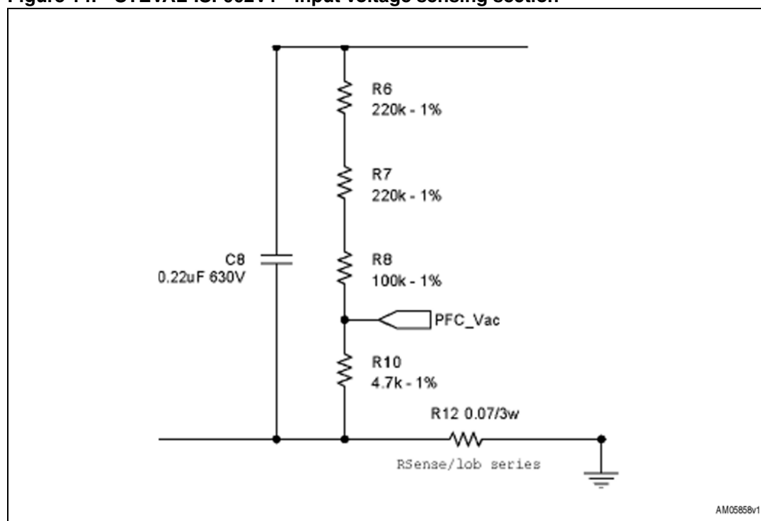
Figure 15. STEVAL-IHM022V1 - input voltage sensing section
