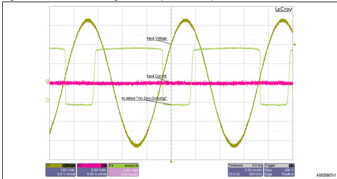
Figure 23. Vin zero crossing detection (without load)
