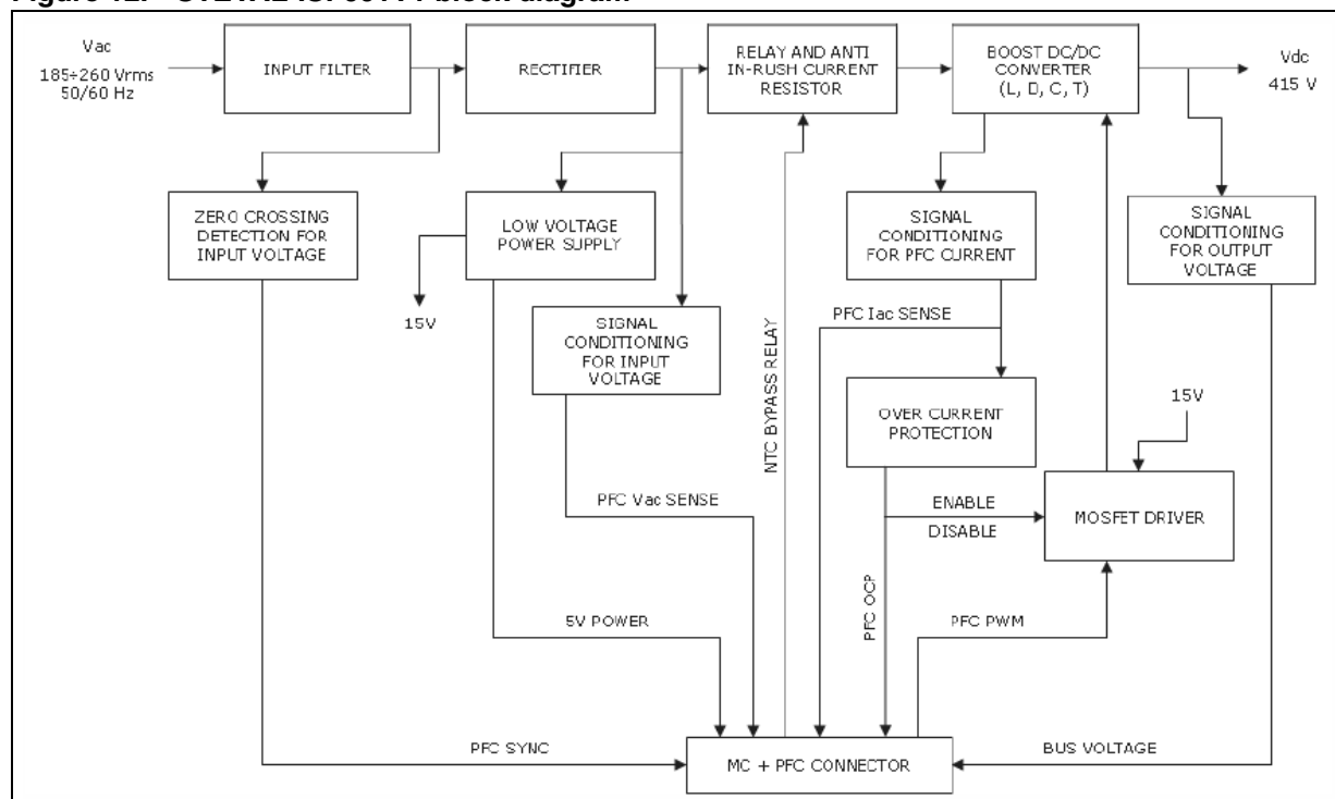
Figure 12. STEVAL-ISF001V1 block diagram
