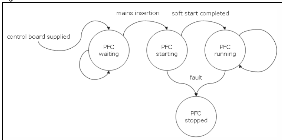
Figure 27. PFC states
