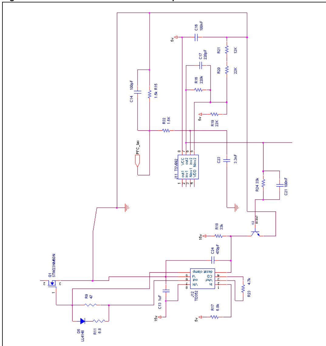
Figure 21. STEVAL-ISF002V1 - overcurrent protection section
