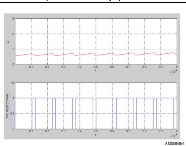
Figure 4. AC to DC boost converter signals with CCM PFC - inductor current and power MOSFET gate command (time scale = 10 \mu s)
