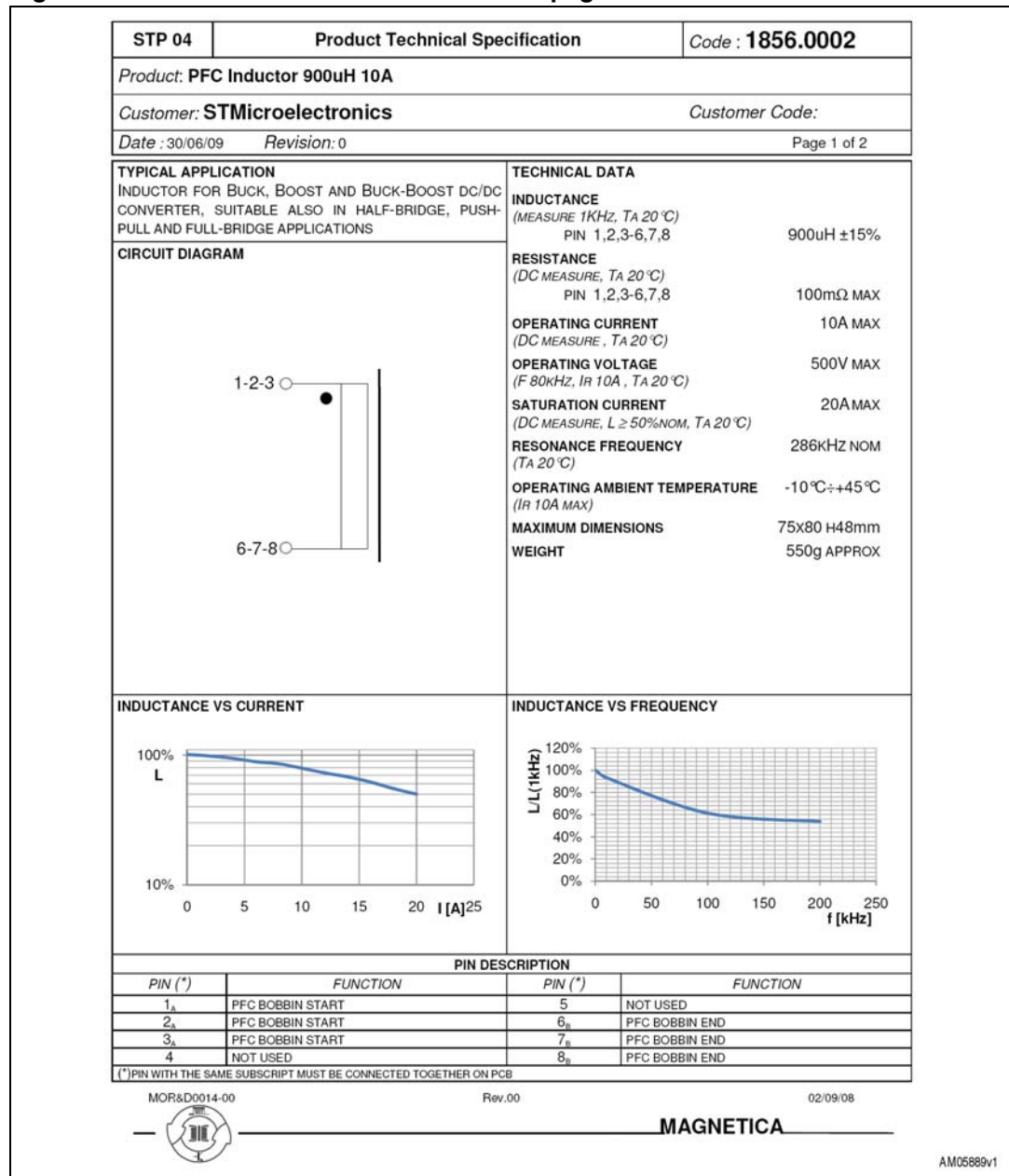
Figure 45. Technical sheet of PFC inductor - page 1 of 2
