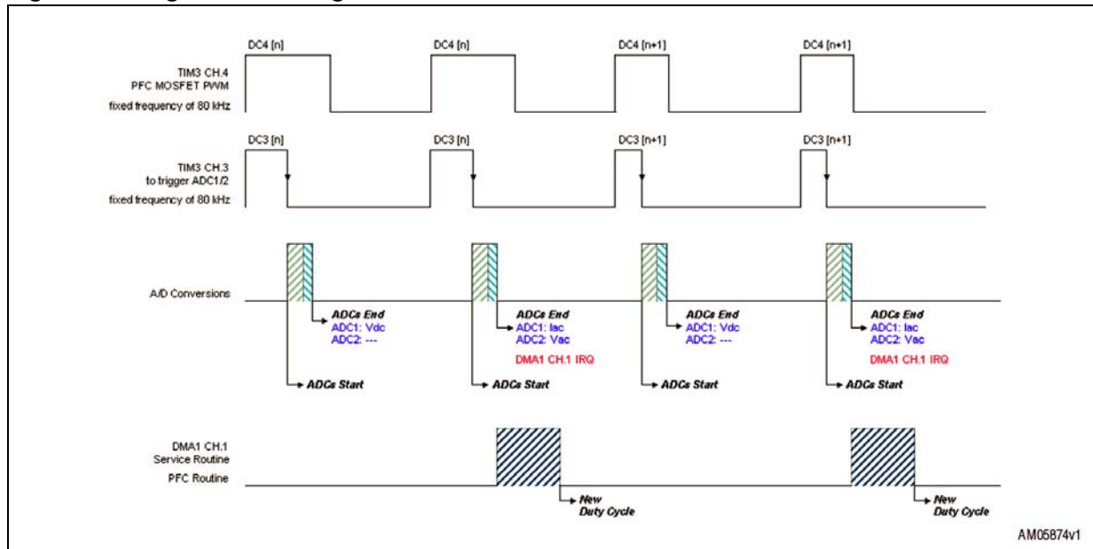
Figure 30. Digital PFC timing
