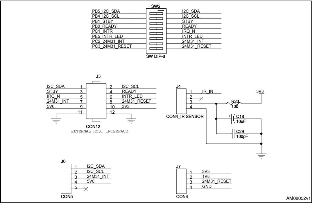
Figure 16. Connectors section
