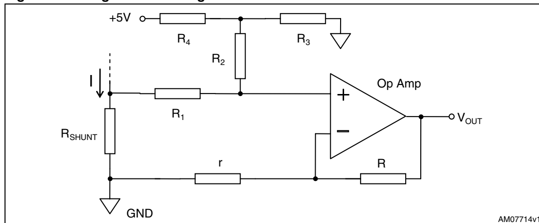
Figure 12. Single-shunt configuration
