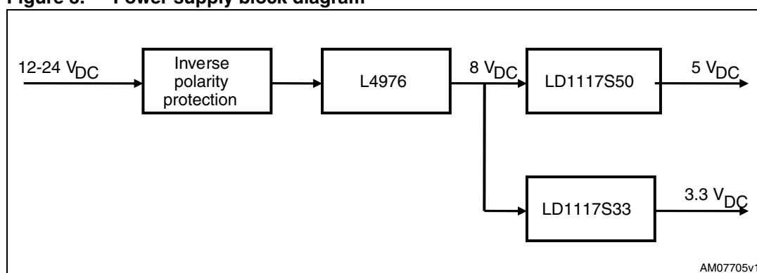
Figure 3. Power supply block diagram
