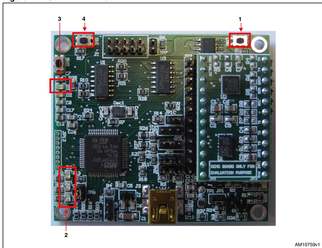
Figure 2. STEVAL-MKI119V1
