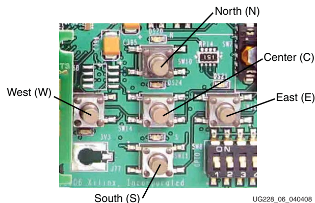
Figure 6: User Pushbuttons
