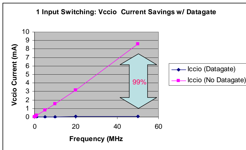
Figure 5: V_{CCIO} Current Savings, Single Input Switching
