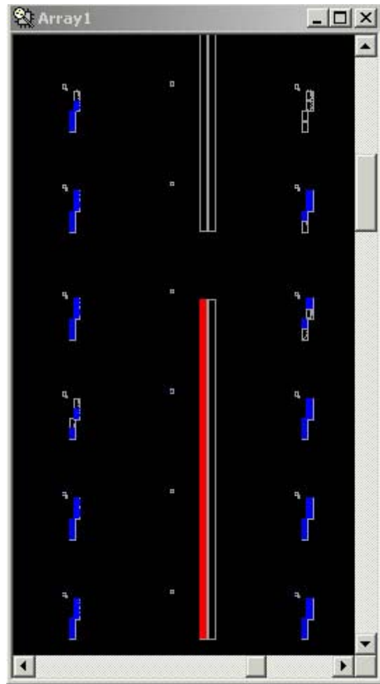
Figure 6: Selected Block
