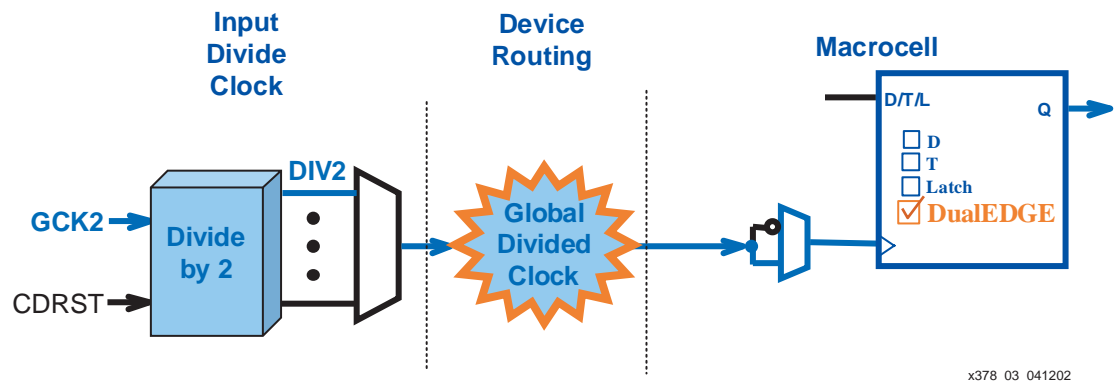
Figure 3: CoolCLOCK
