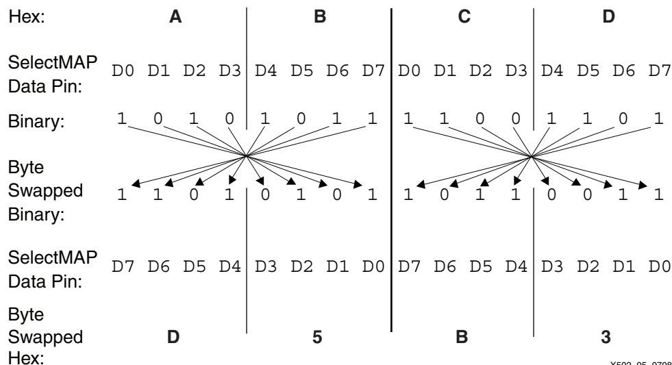
Figure 3: Byte-Swapping Example
