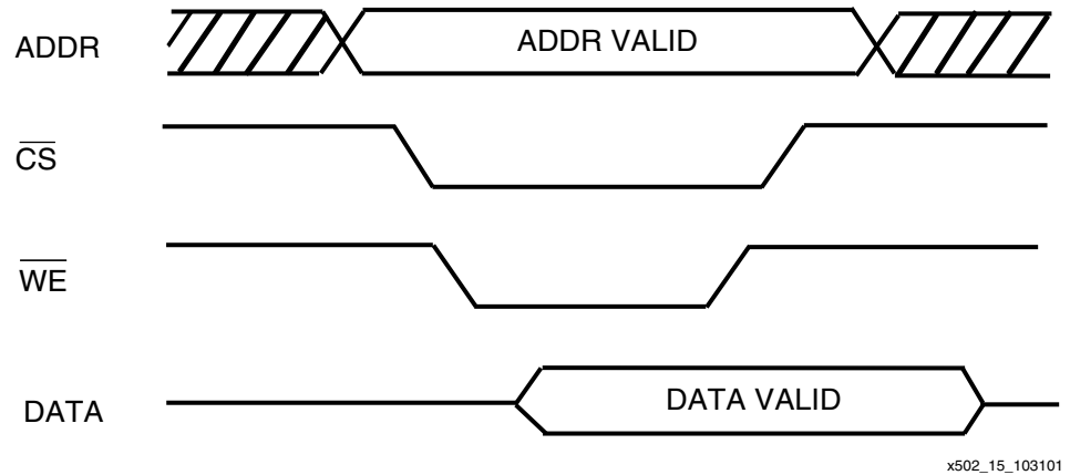
Figure 12: Write-Cycle Timing Diagram
