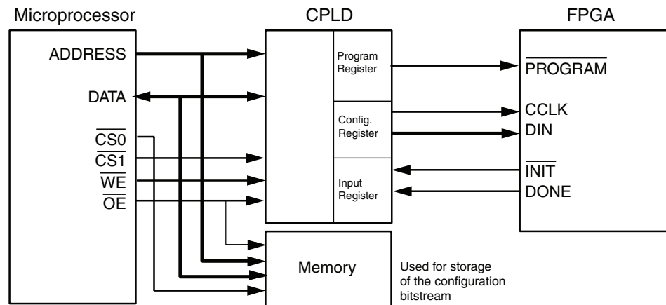
Figure 9: Slave Serial Configuration
