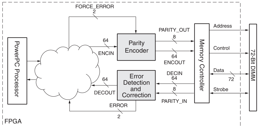
Figure 5: ECC in a Memory System
