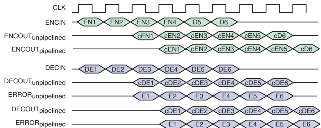
Figure 8: Timing Diagram
