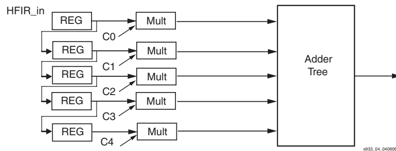
Figure 4: Horizontal FIR
