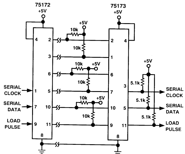
Figure 4. AD2S90 RS-485 Communication
