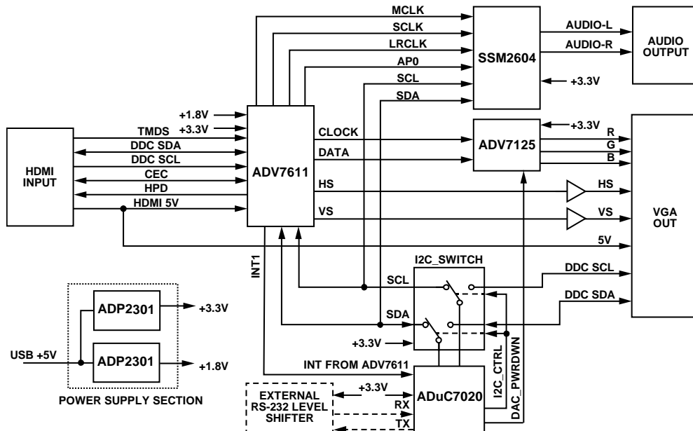
Figure 1. HDMI-to-VGA (HDMI2VGA) Converter Block Diagram (Simplified Schematic: All Connections Not Shown)
