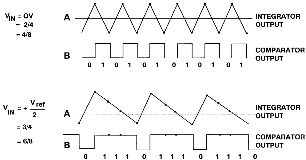
Figure 5: Sigma-Delta Modulator Waveforms
