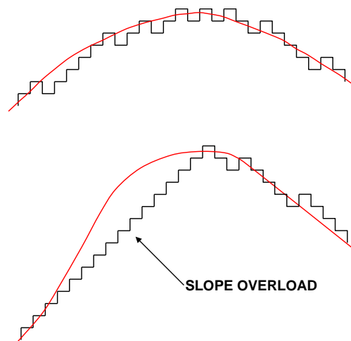
Figure 2: Quantization Using Delta Modulation
