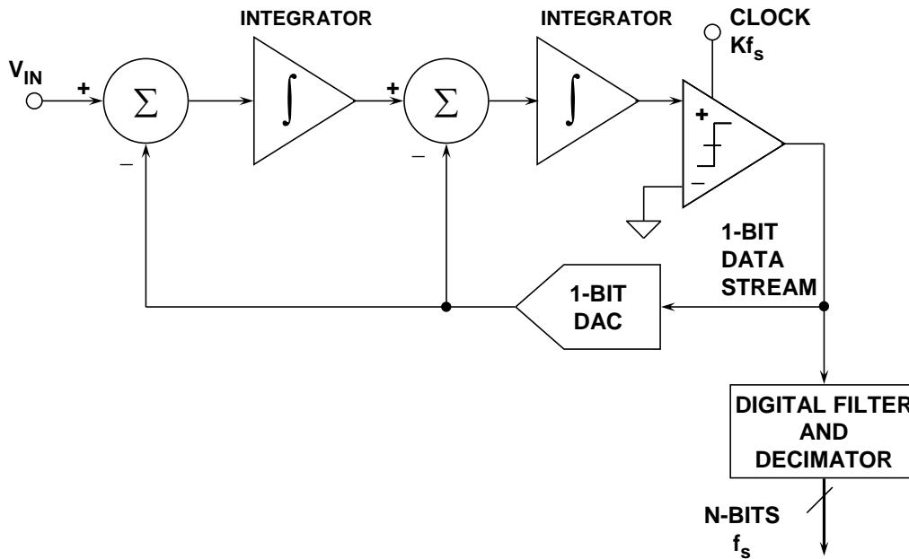
Figure 8: Second-Order Sigma-Delta ADC
