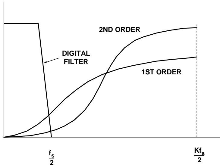
Figure 7: Sigma-Delta Modulators Shape Quantization Noise
