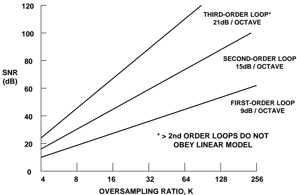
Figure 9: SNR Versus Oversampling Ratio for First, Second, and Third-Order Loops
