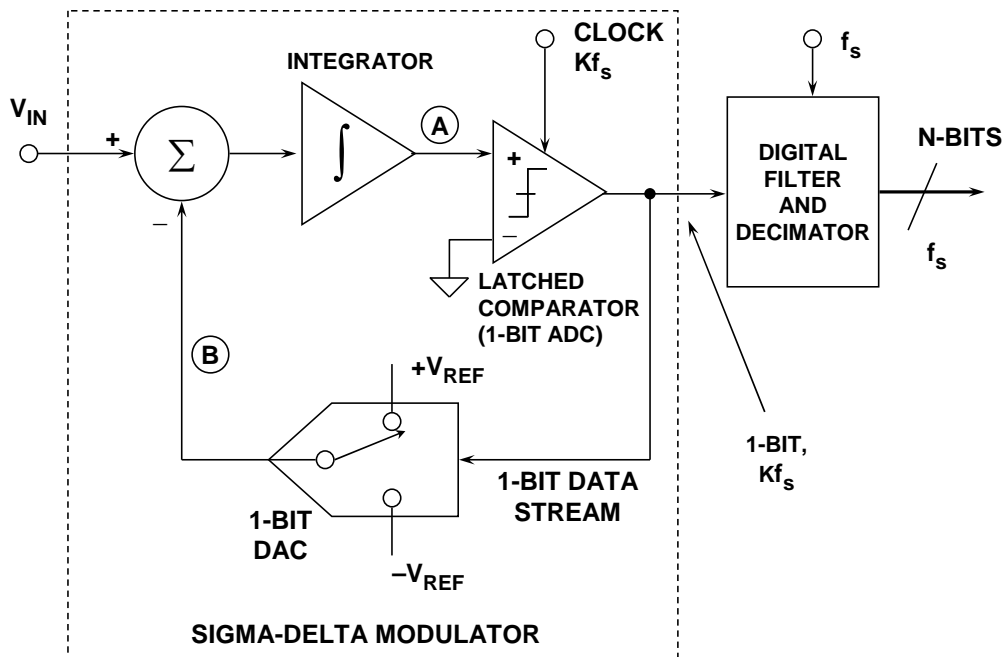
Figure 4: First-Order Sigma-Delta ADC
