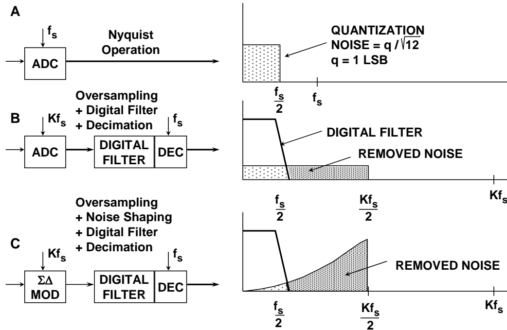
Figure 3: Oversampling, Digital Filtering, Noise Shaping, and Decimation
