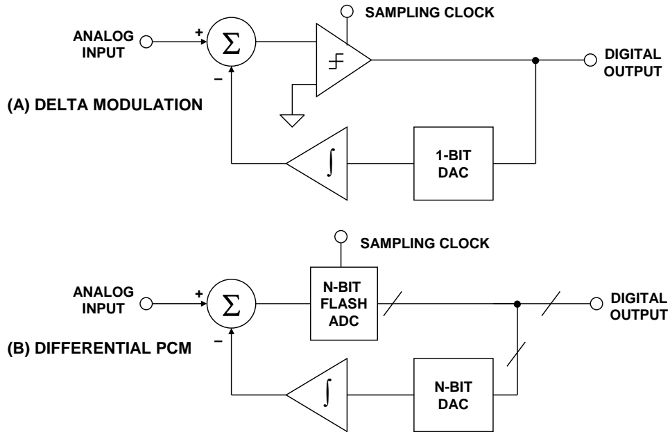
Figure 1: Delta Modulation and Differential PCM
