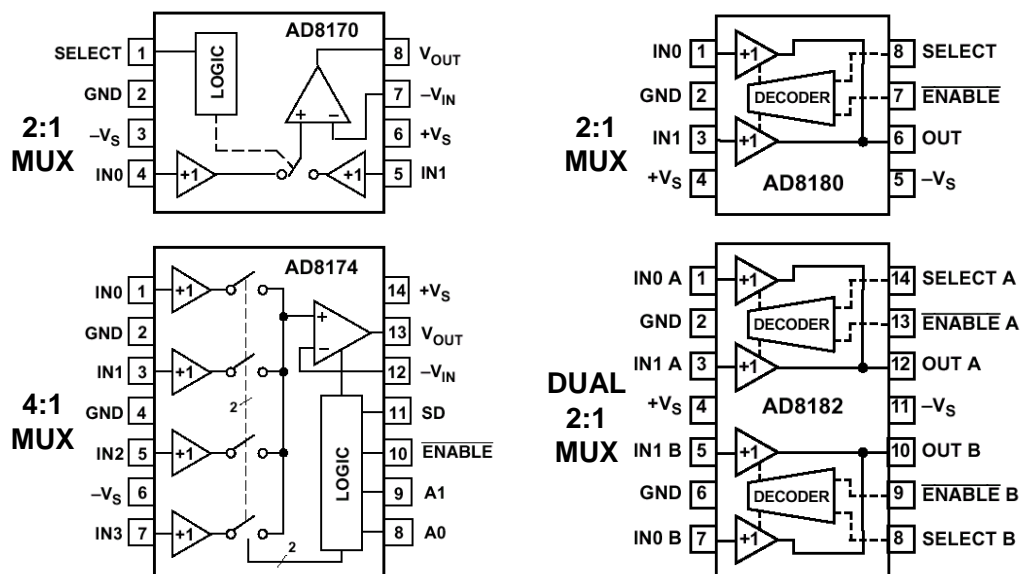
Figure 1: AD8170/8174/8180/8182 Bipolar Video Multiplexers
