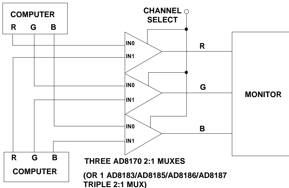
Figure 3: Dual Source RGB Multiplexer Using Three 2:1 Muxes
