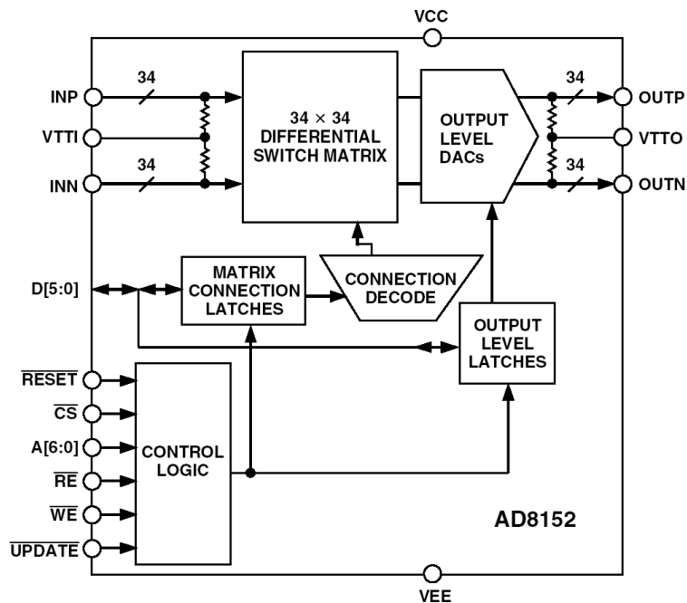
Figure 6: AD8152 3.2-Gbps Asynchronous Digital Crosspoint Switch
