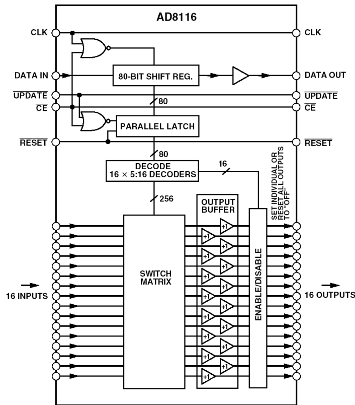
Figure 5: AD8116 16x16 200-MHz Buffered Video Crosspoint Switch
