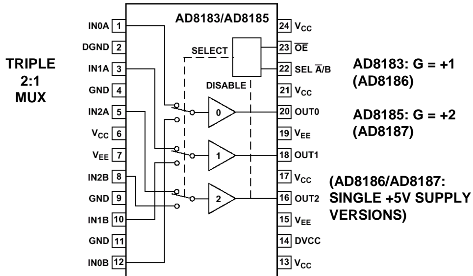
Figure 2: AD8183/AD8185 Triple 2:1 Video Multiplexers
