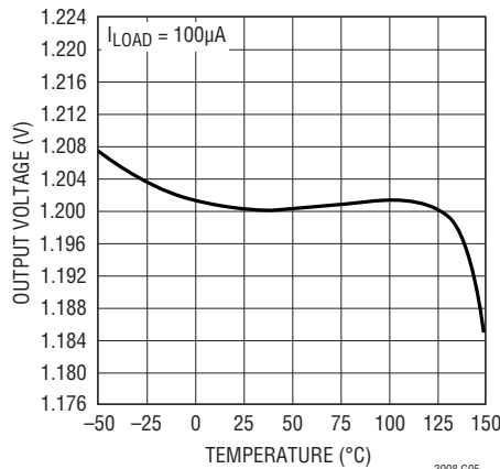
Output Voltage LT3008-1.2
