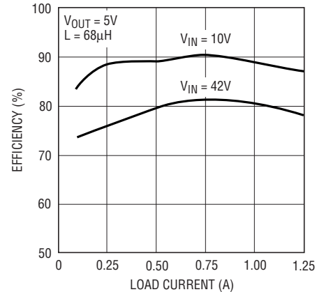
Buck Converter Efficiency vs Load Current
